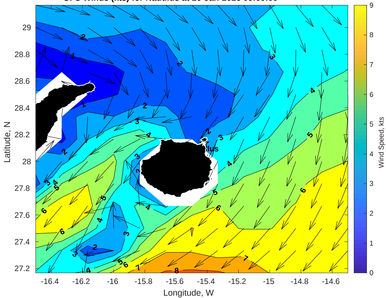
GFS Winds (kts) for Nautilus at 26-Jan-2026 09:00:00
