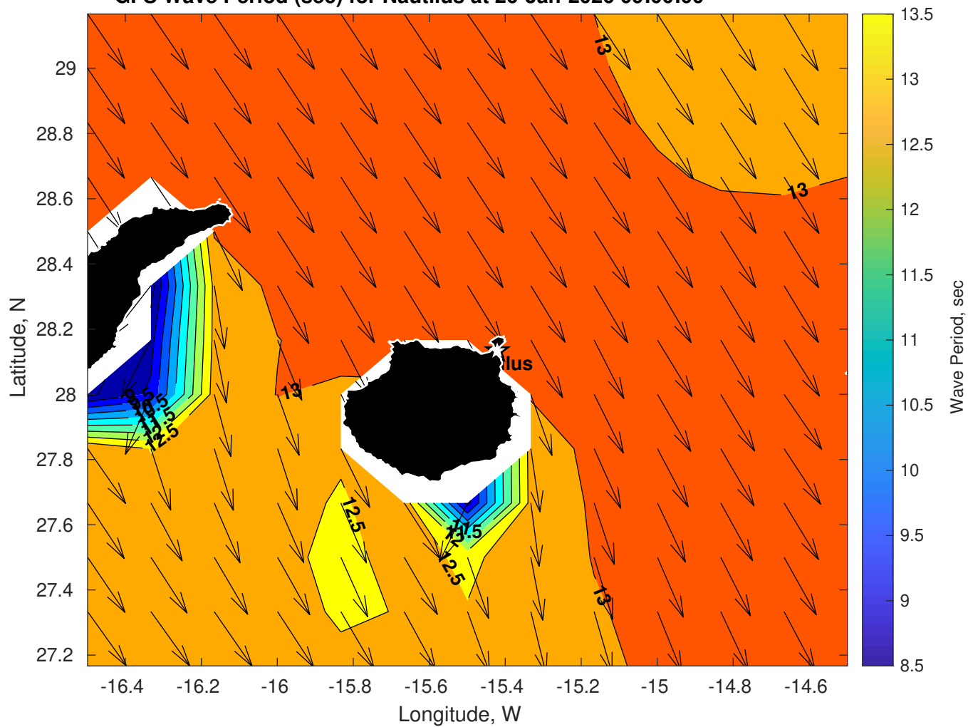
GFS Wave Period (sec) for Nautilus at 26-Jan-2026 09:00:00
