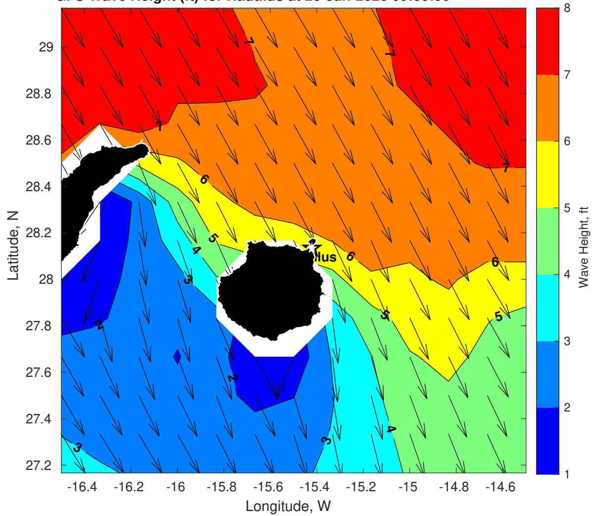
GFS Wave Height (ft) for Nautilus at 26-Jan-2026 09:00:00
