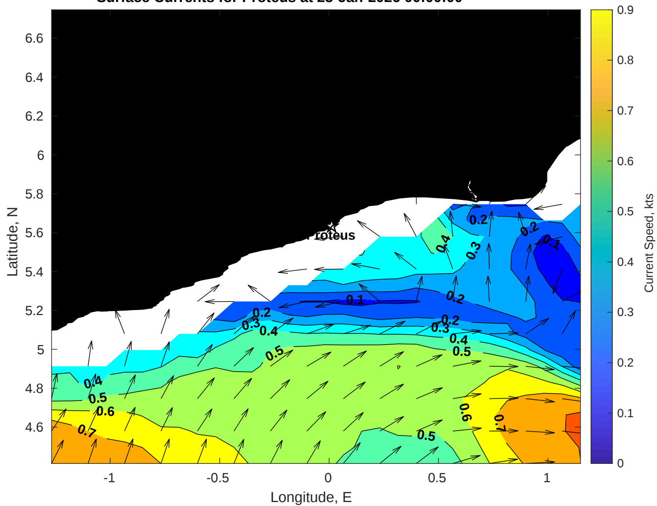
Surface Currents for Proteus at 25-Jan-2026 00:00:00
