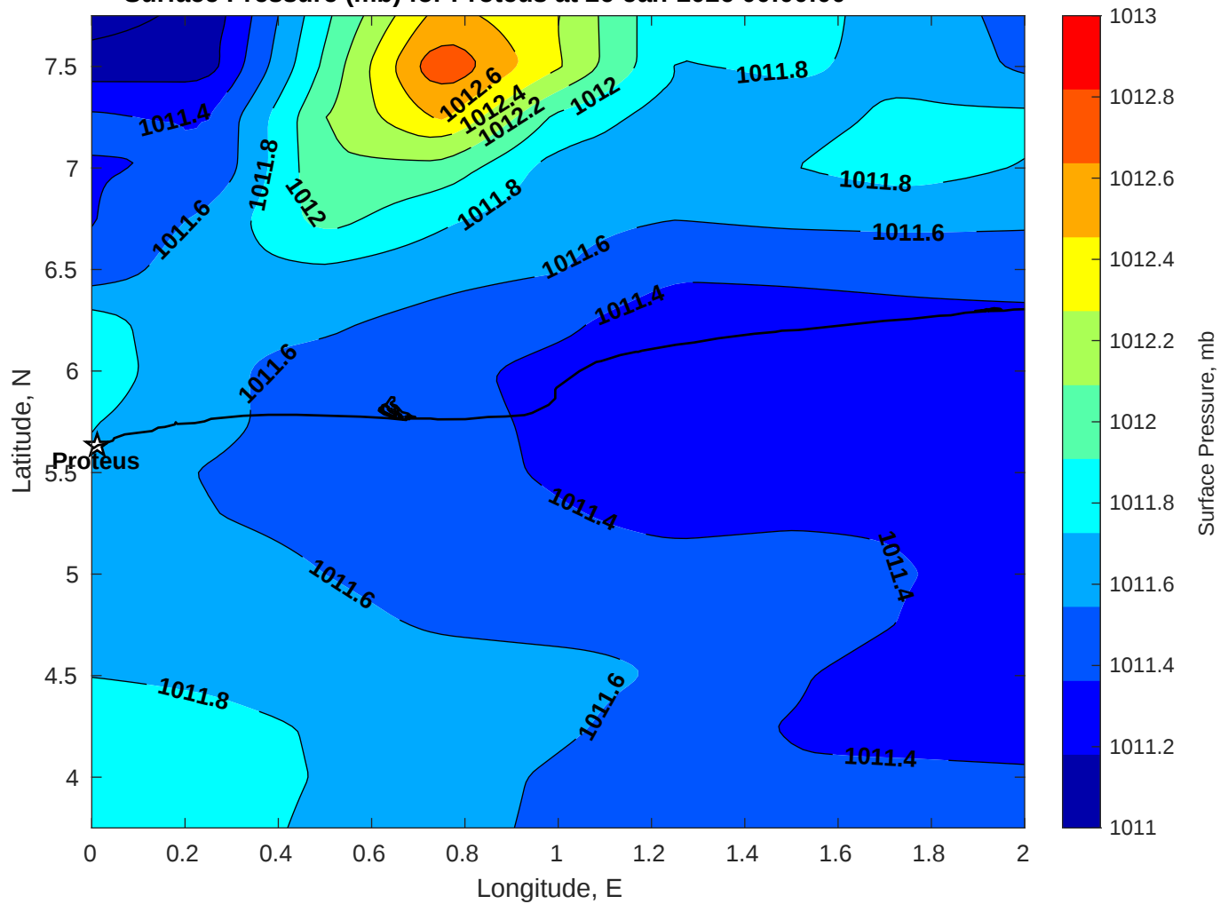
Surface Pressure (mb) for Proteus at 26-Jan-2026 00:00:00
