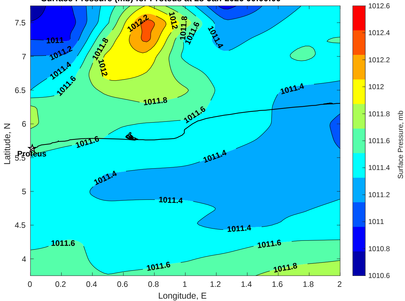
Surface Pressure (mb) for Proteus at 28-Jan-2026 00:00:00
