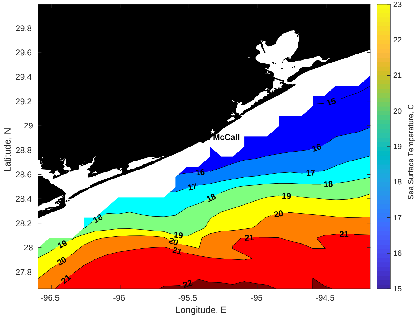
SST for Brooks McCall at 26-Jan-2026 00:00:00
