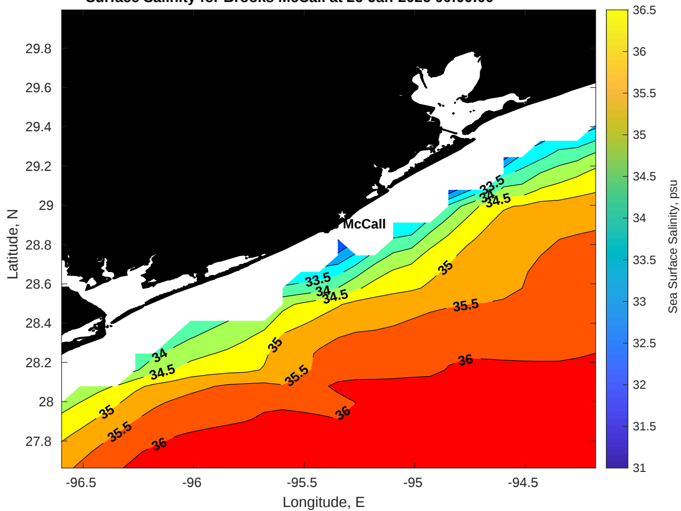
Surface Salinity for Brooks McCall at 26-Jan-2026 00:00:00
