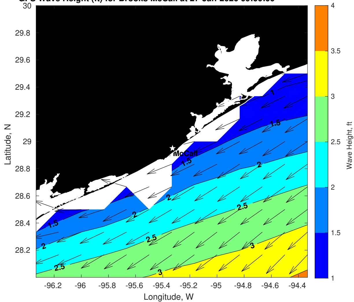
GFS Wave Height (ft) for Brooks McCall at 27-Jan-2026 09:00:00
