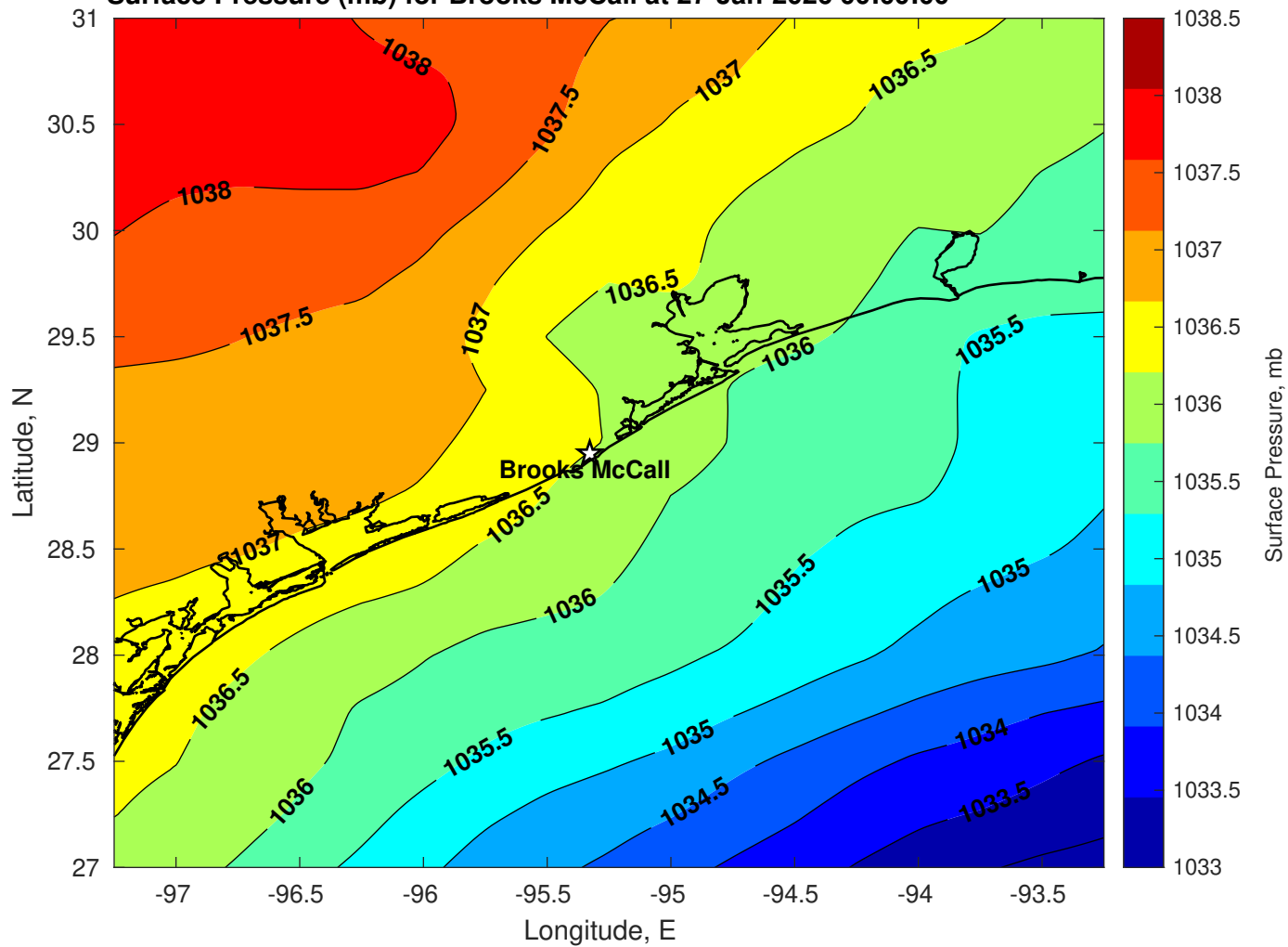
Surface Pressure (mb) for Brooks McCall at 27-Jan-2026 00:00:00
