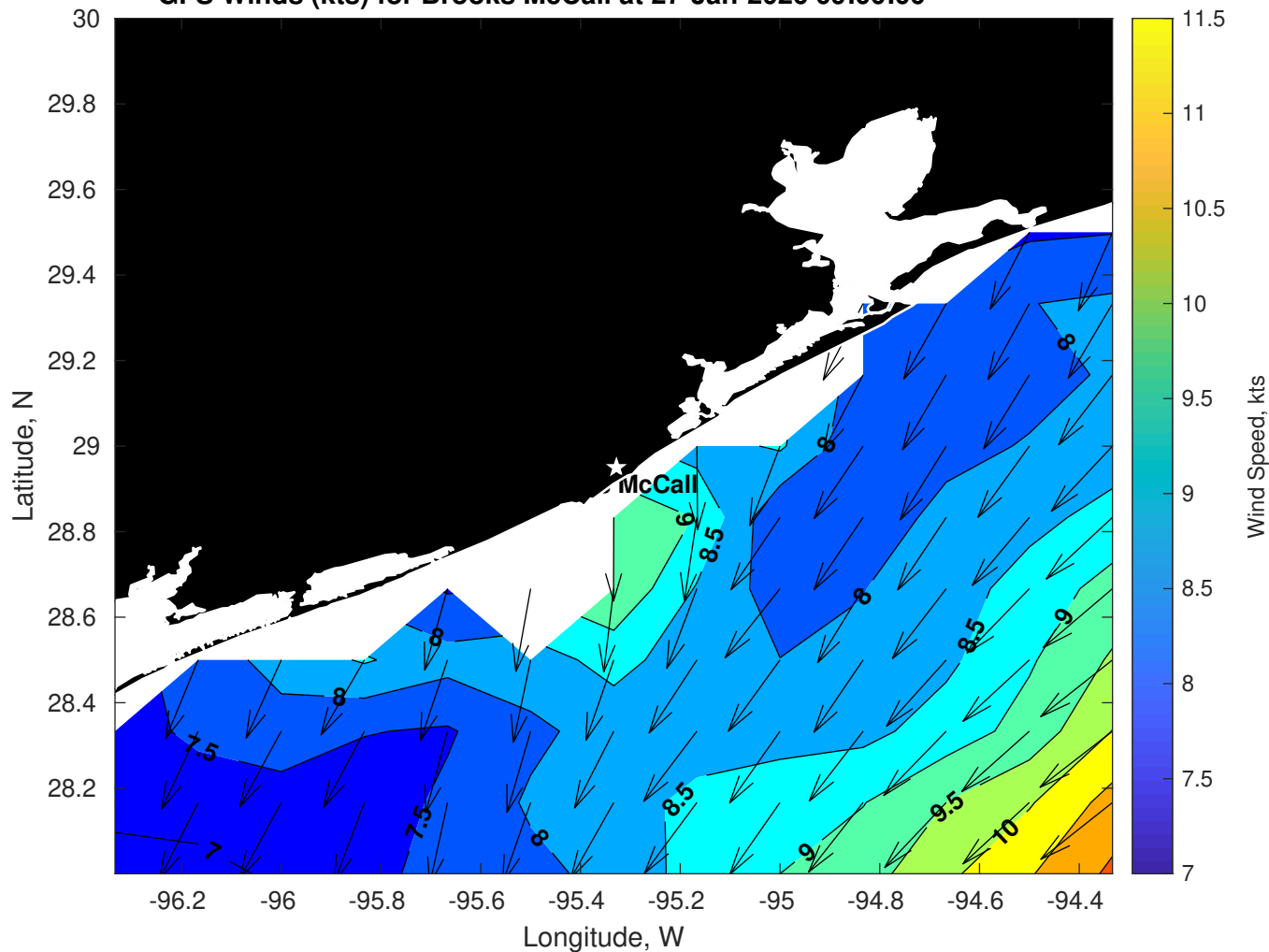
GFS Winds (kts) for Brooks McCall at 27-Jan-2026 09:00:00
