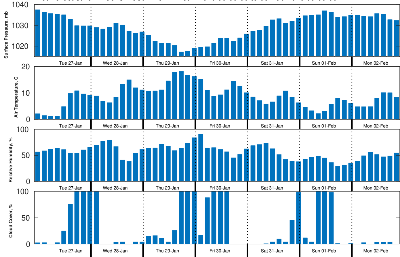
Met Forecast for Brooks McCall from 27-Jan-2026 00:00:00 to 03-Feb-2026 00:00:00
