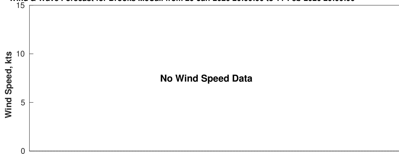
Wind & Wave Forecast for Brooks McCall from 26-Jan-2026 20:00:00 to 11-Feb-2026 20:00:00
