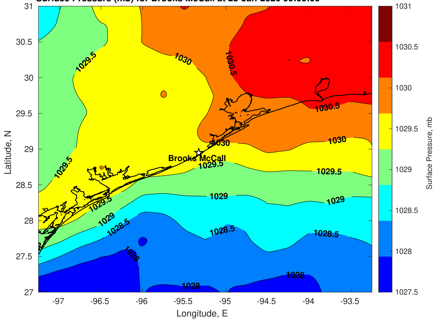
Surface Pressure (mb) for Brooks McCall at 28-Jan-2026 00:00:00
