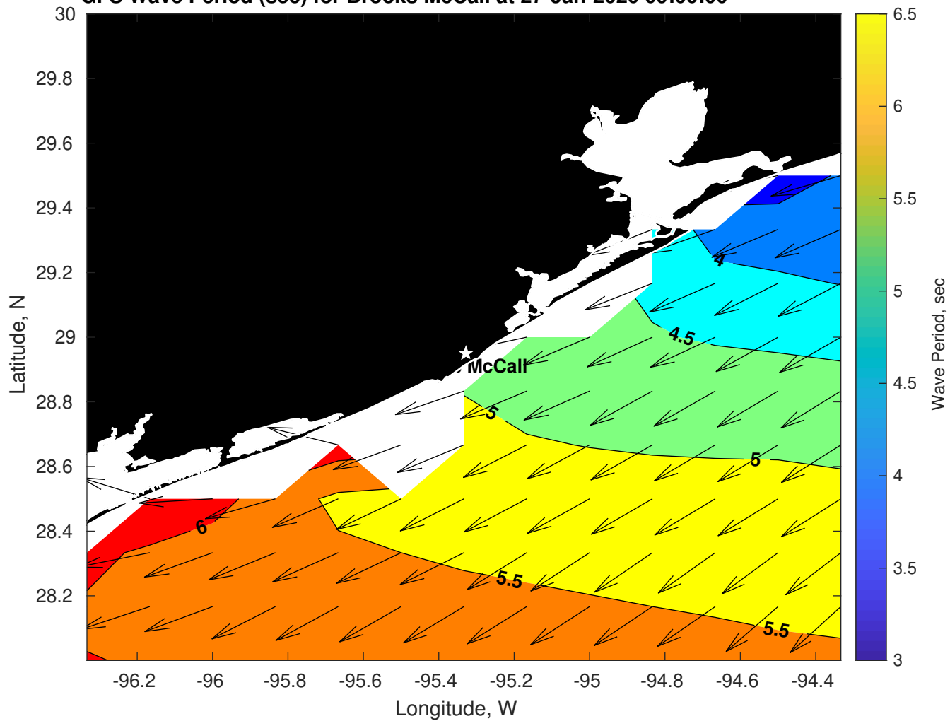
GFS Wave Period (sec) for Brooks McCall at 27-Jan-2026 09:00:00
