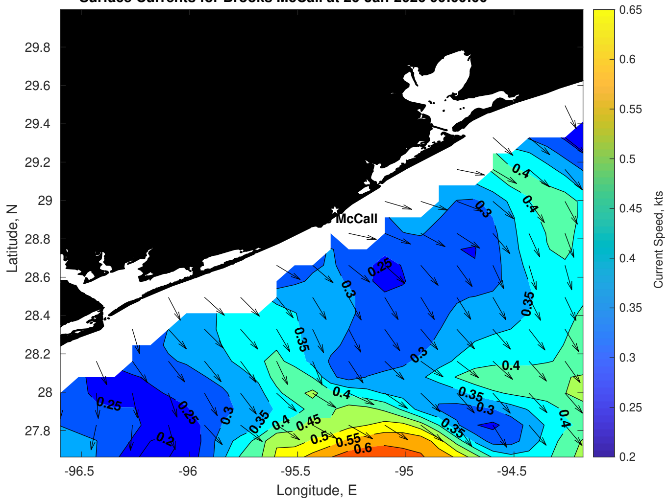
Surface Currents for Brooks McCall at 26-Jan-2026 00:00:00
