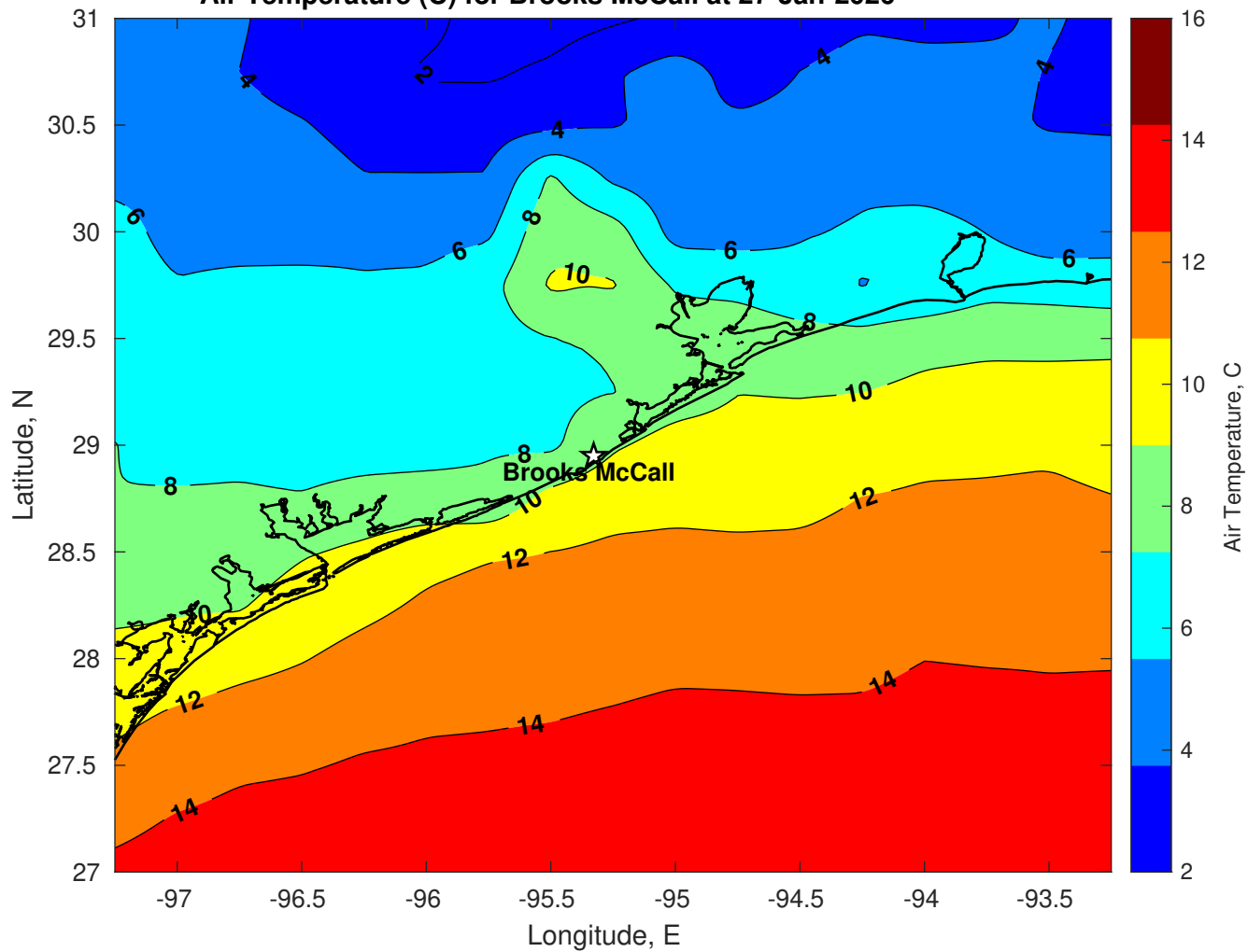
Air Temperature (C) for Brooks McCall at 27-Jan-2026
