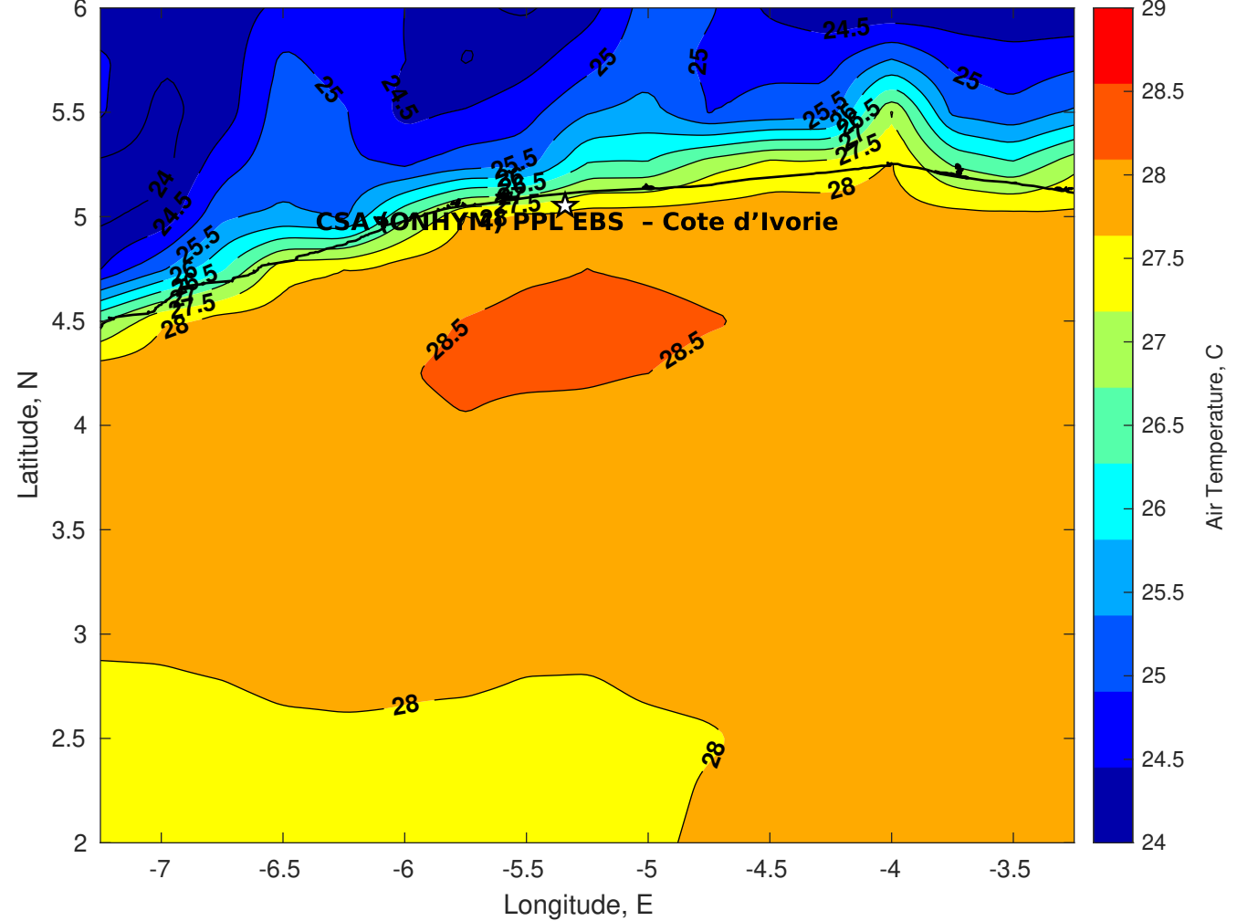
Air Temperature (C) for CSA (ONHYM) PPL EBS - Cote d'Ivoire at 27-Jan-2026
