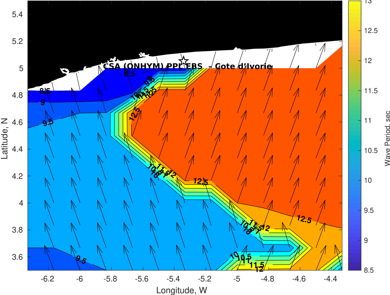
GFS Wave Period (sec) for CSA (ONHYM) PPL EBS - Cote d'Ivoire at 27-Jan-2026 09:00:00
