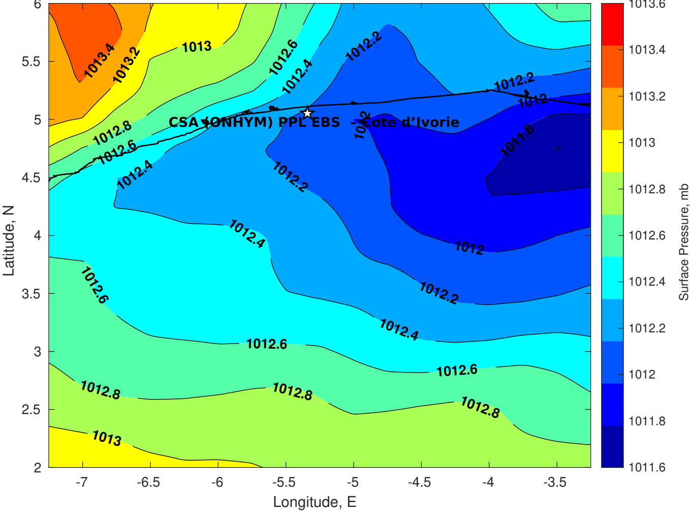
Surface Pressure (mb) for CSA (ONHYM) PPL EBS - Cote d'Ivoire at 28-Jan-2026 00:00:00
