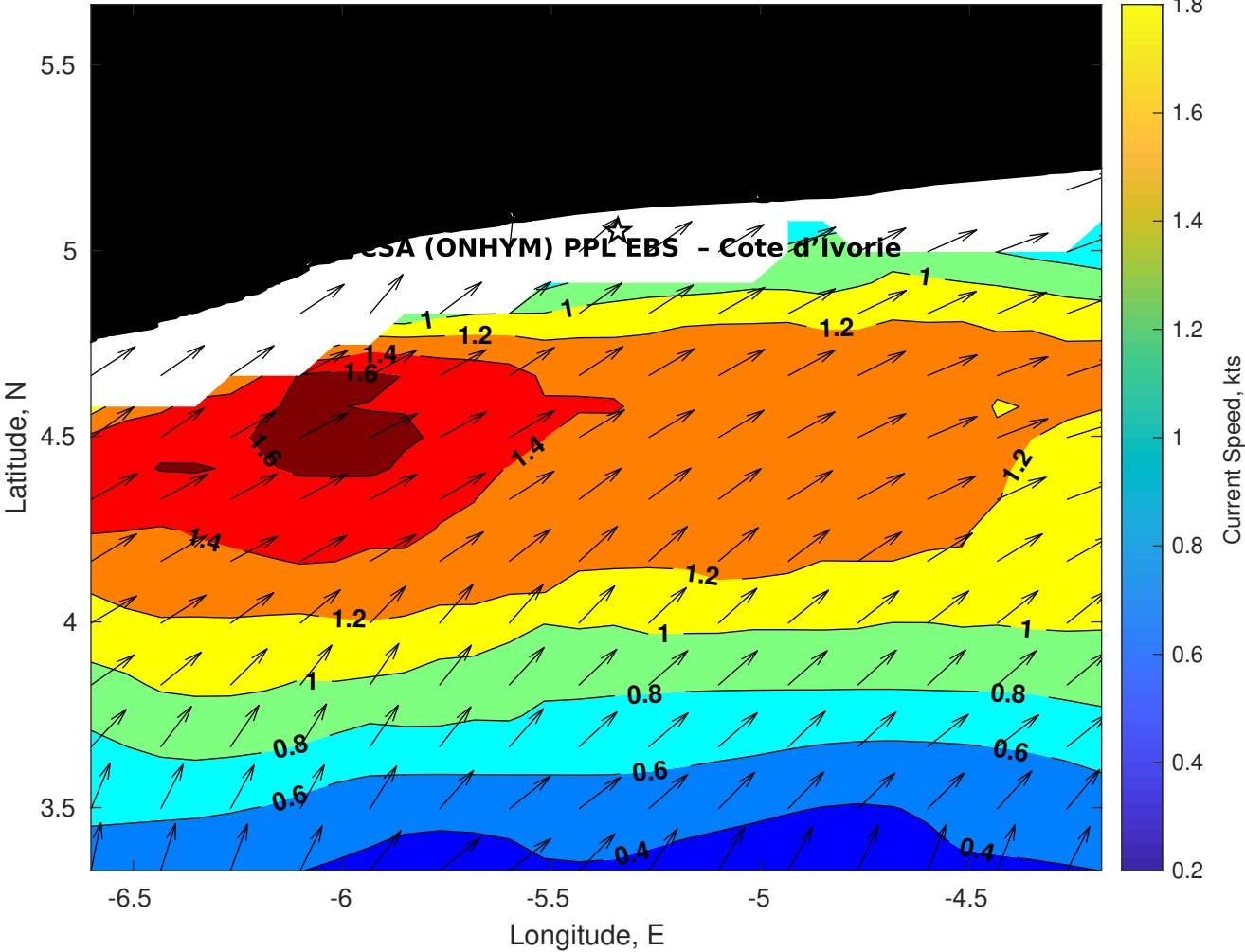
Surface Currents for CSA (ONHYM) PPL EBS - Cote d'Ivoire at 26-Jan-2026 00:00:00
