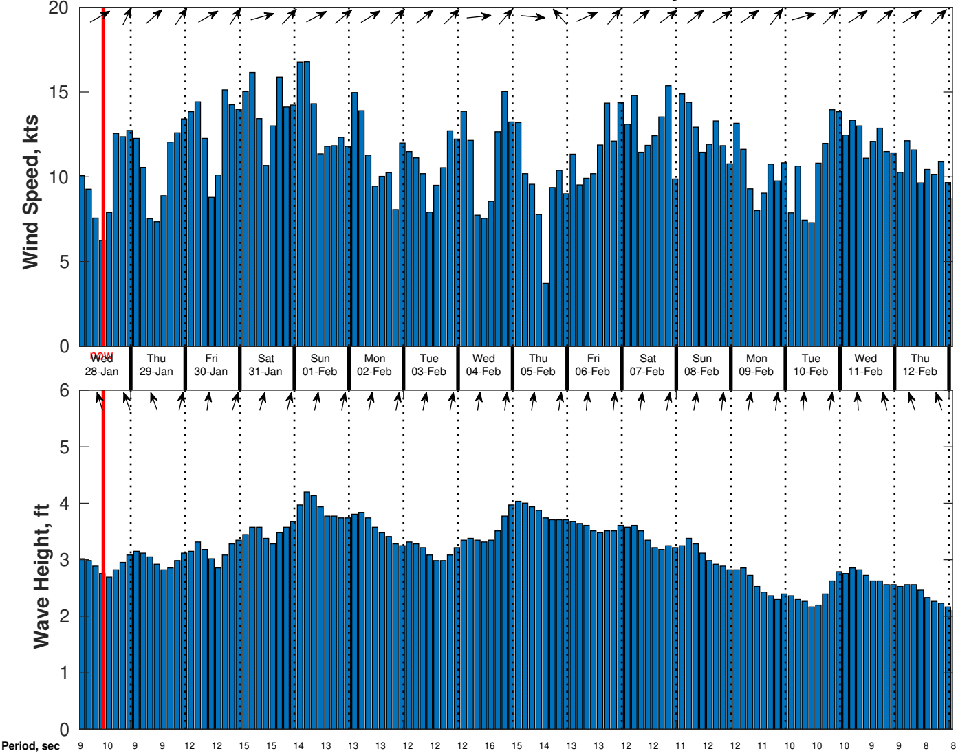
Wind & Wave Forecast for CSA (ONHYM) PPL EBS - Cote d'Ivoire from 27-Jan-2026 01:00:00 to 12-Feb-2026 01:00:00
