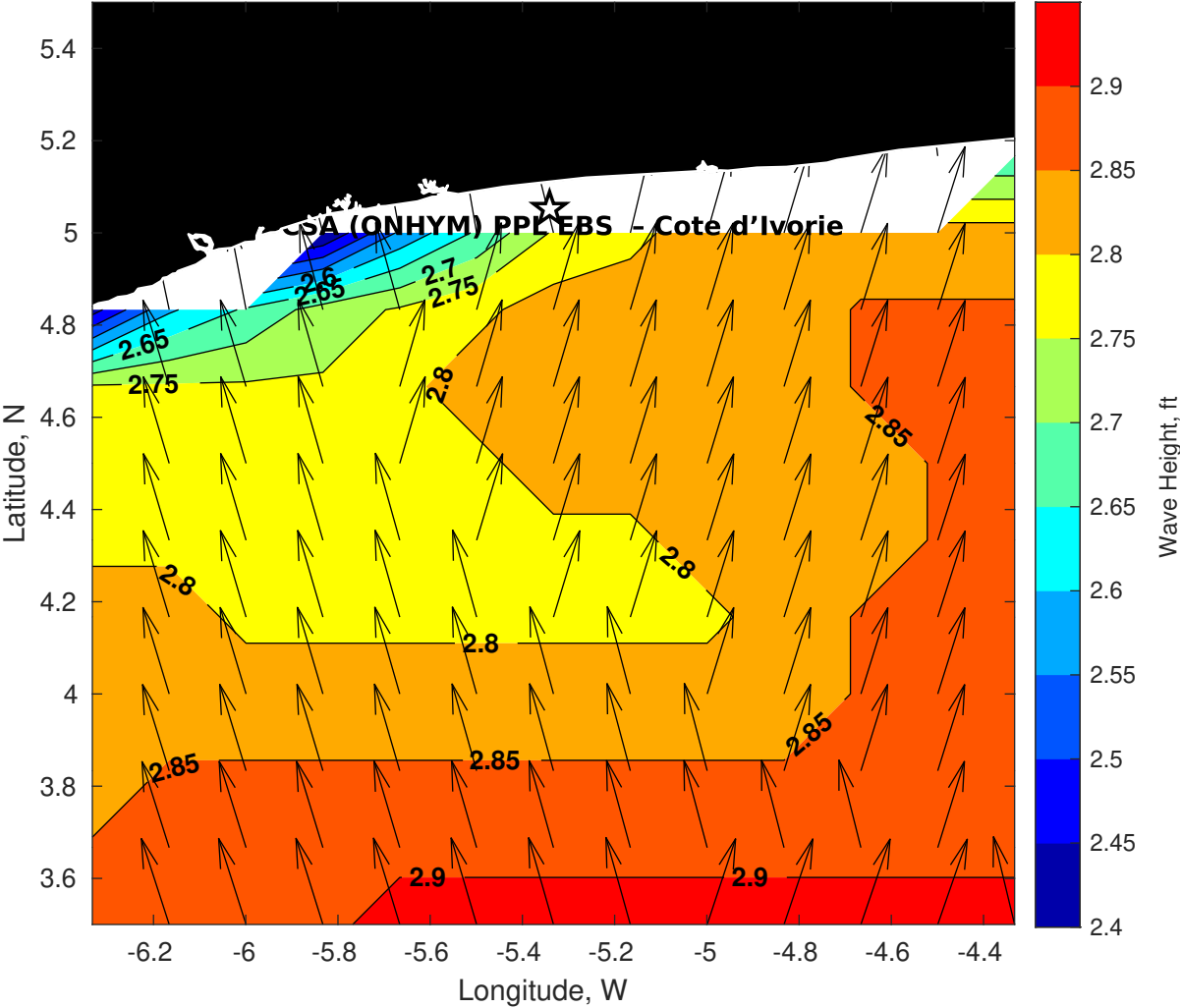
GFS Wave Height (ft) for CSA (ONHYM) PPL EBS - Cote d'Ivoire at 27-Jan-2026 09:00:00
