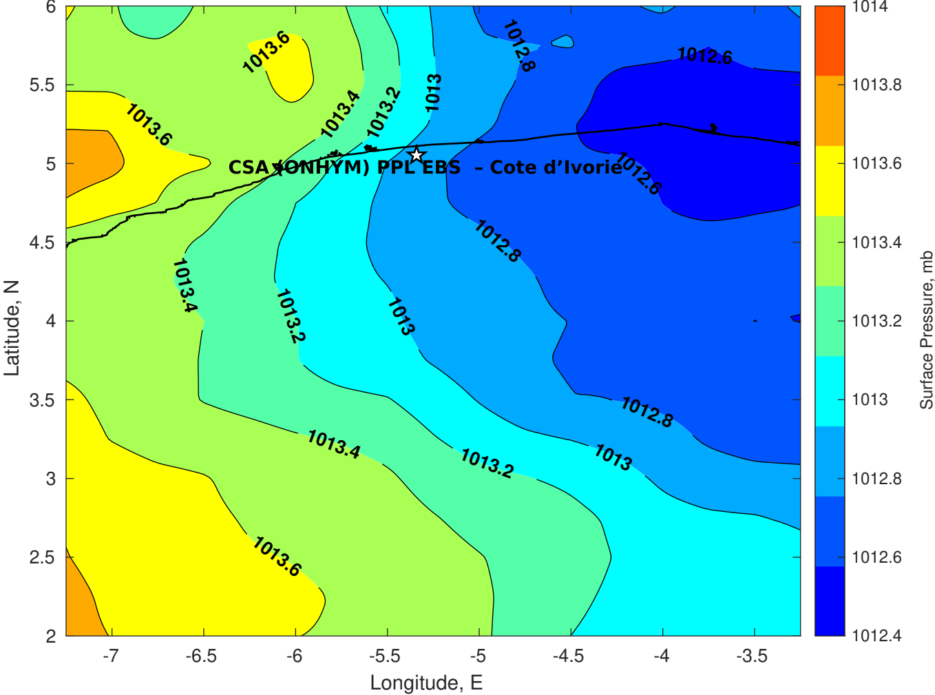
Surface Pressure (mb) for CSA (ONHYM) PPL EBS - Cote d'Ivoire at 29-Jan-2026 00:00:00
