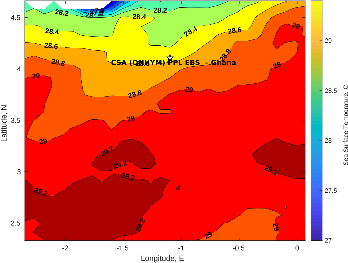
SST for CSA (ONHYM) PPL EBS - Ghana at 26-Jan-2026 00:00:00
