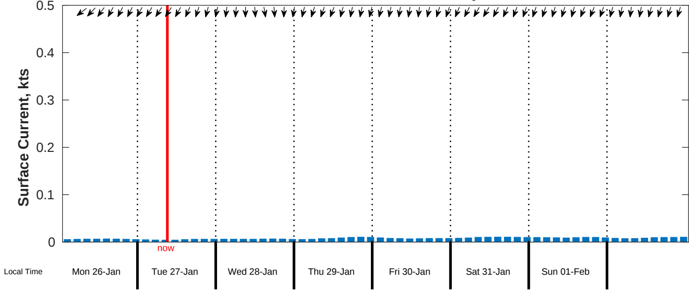
Surface Current Forecast for CSA (ONHYM) PPL EBS - Ghana from 26-Jan-2026 00:00:00 to 03-Feb-2026 00:00:00
