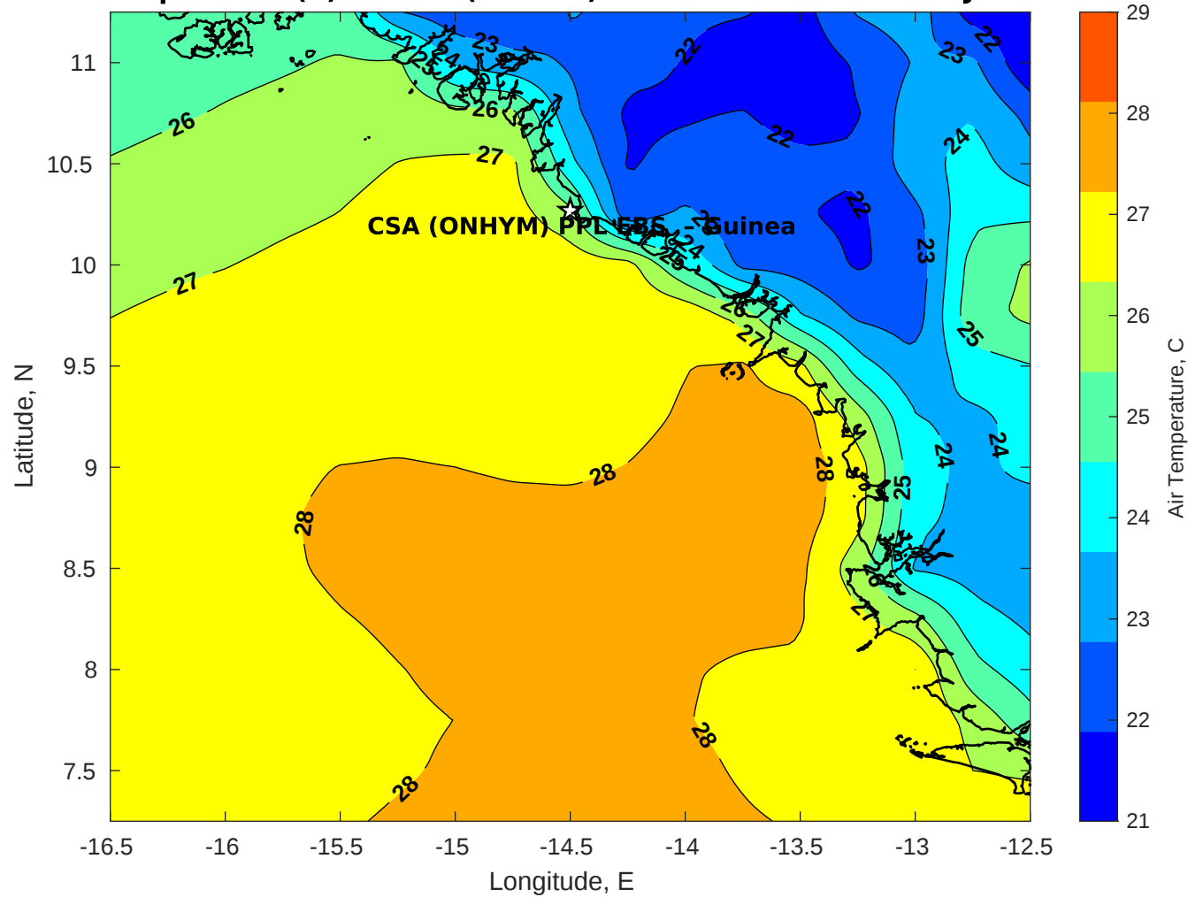
Air Temperature (C) for CSA (ONHYM) PPL EBS - Guinea at 27-Jan-2026
