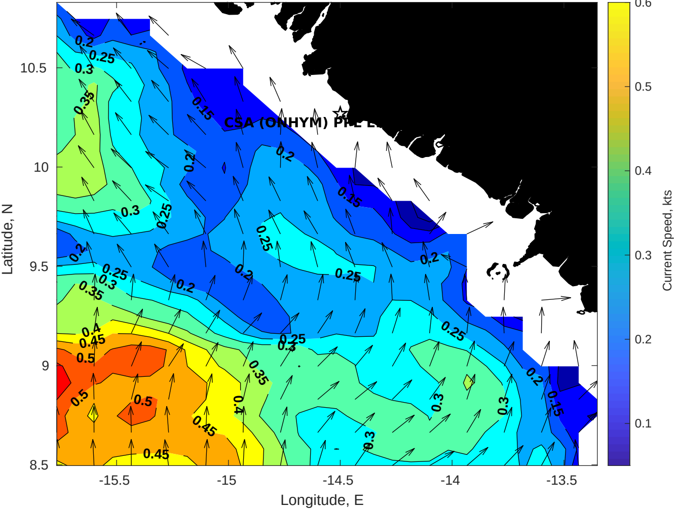
Surface Currents for CSA (ONHYM) PPL EBS - Guinea at 26-Jan-2026 00:00:00
