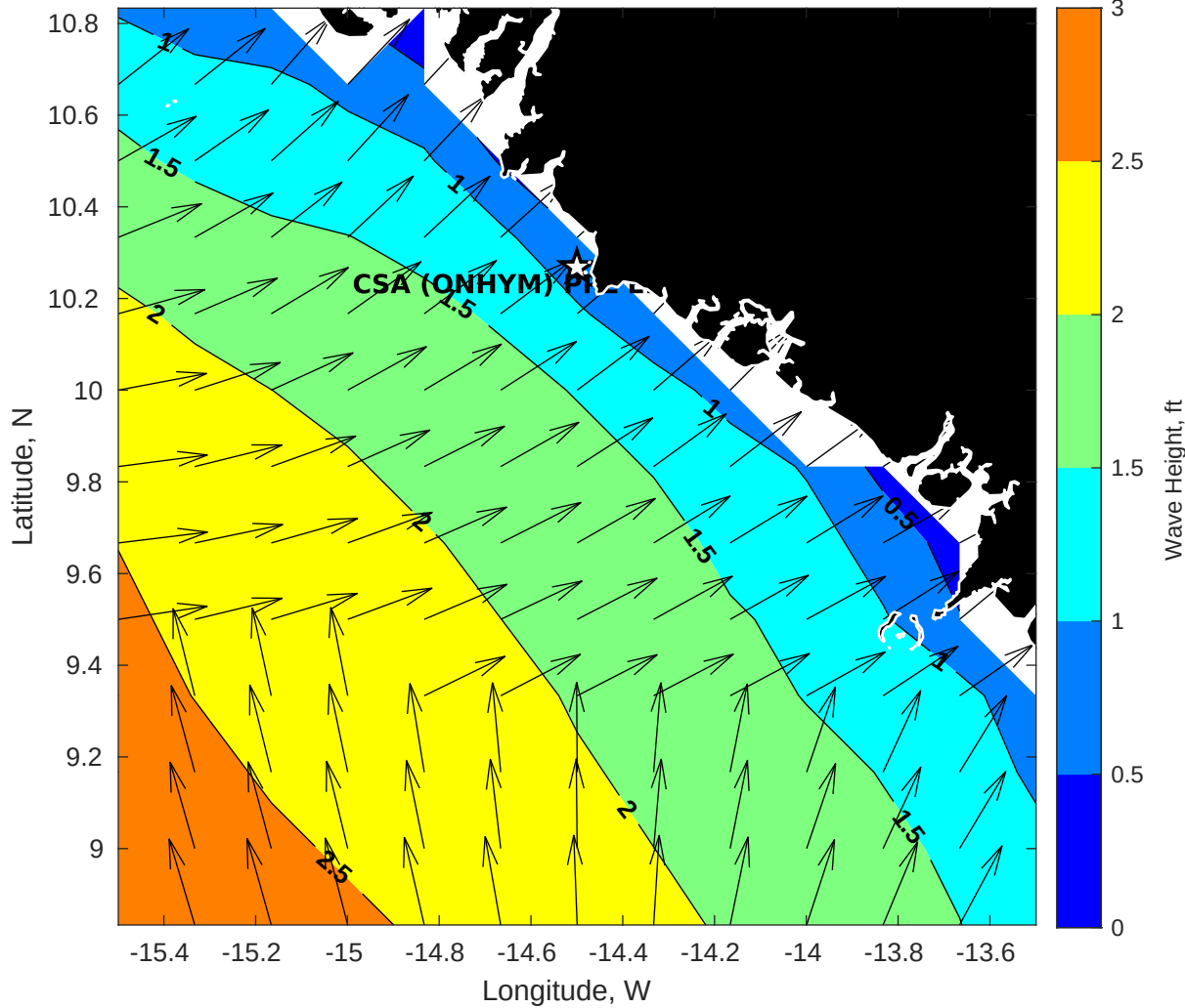
GFS Wave Height (ft) for CSA (ONHYM) PPL EBS - Guinea at 27-Jan-2026 09:00:00
