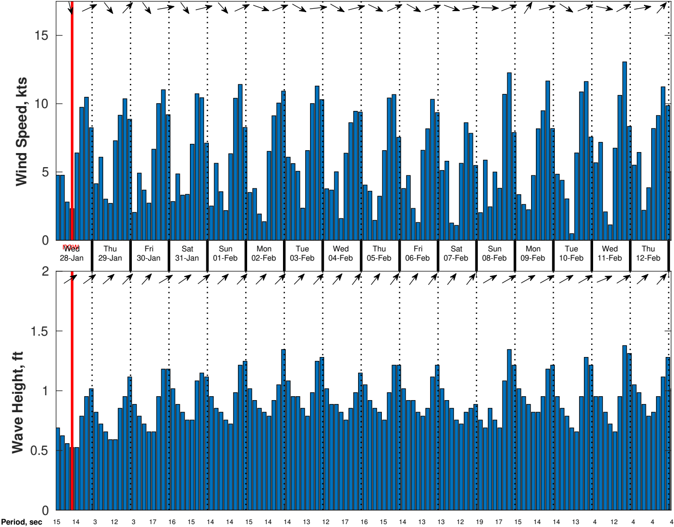
Wind & Wave Forecast for CSA (ONHYM) PPL EBS - Guinea from 27-Jan-2026 01:00:00 to 12-Feb-2026 01:00:00
