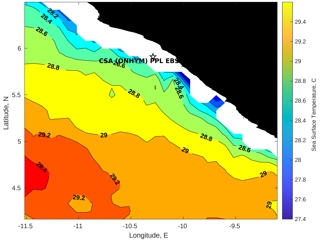
SST for CSA (ONHYM) PPL EBS - Liberia at 26-Jan-2026 00:00:00
