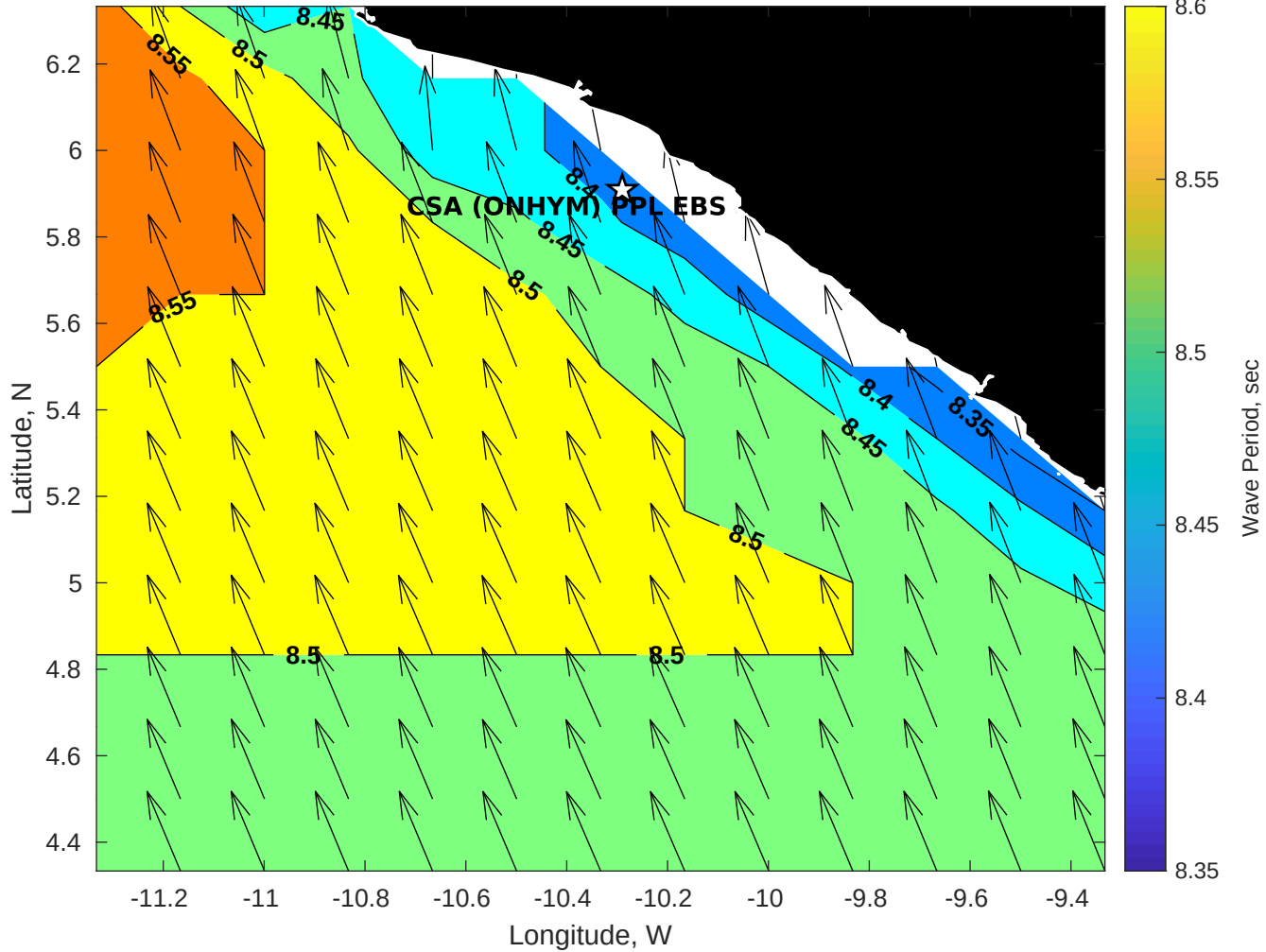
GFS Wave Period (sec) for CSA (ONHYM) PPL EBS - Liberia at 27-Jan-2026 09:00:00
