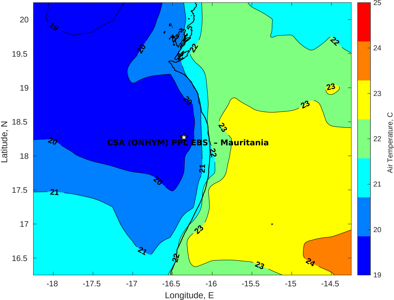
Air Temperature (C) for CSA (ONHYM) PPL EBS - Mauritania at 27-Jan-2026
