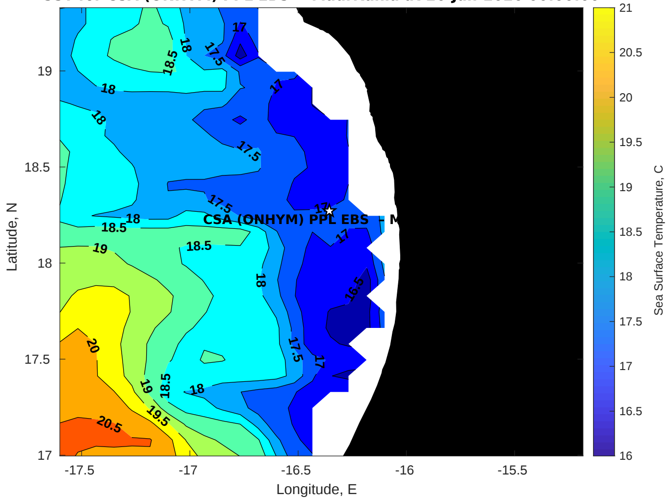
SST for CSA (ONHYM) PPL EBS - Mauritania at 26-Jan-2026 00:00:00
