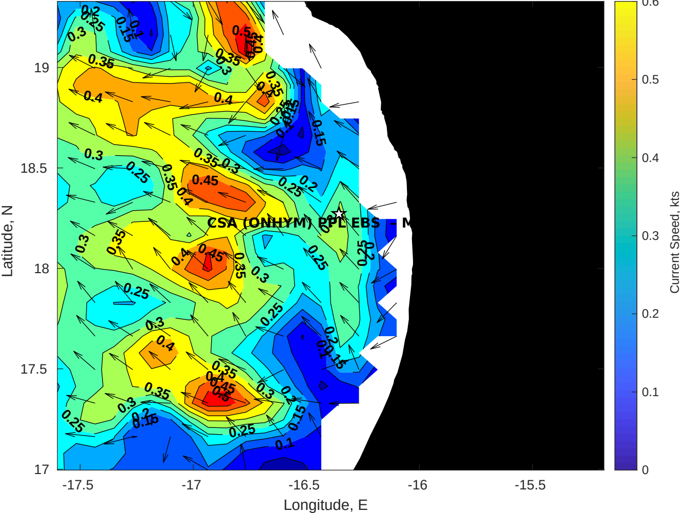
Surface Currents for CSA (ONHYM) PPL EBS - Mauritania at 26-Jan-2026 00:00:00
