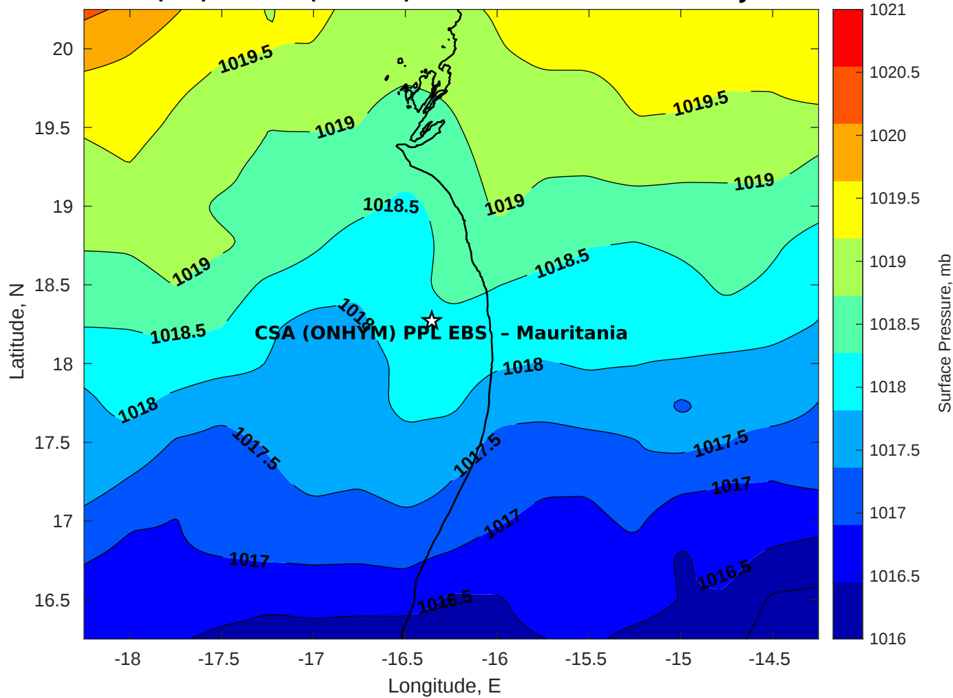
Surface Pressure (mb) for CSA (ONHYM) PPL EBS - Mauritania at 27-Jan-2026 00:00:00
