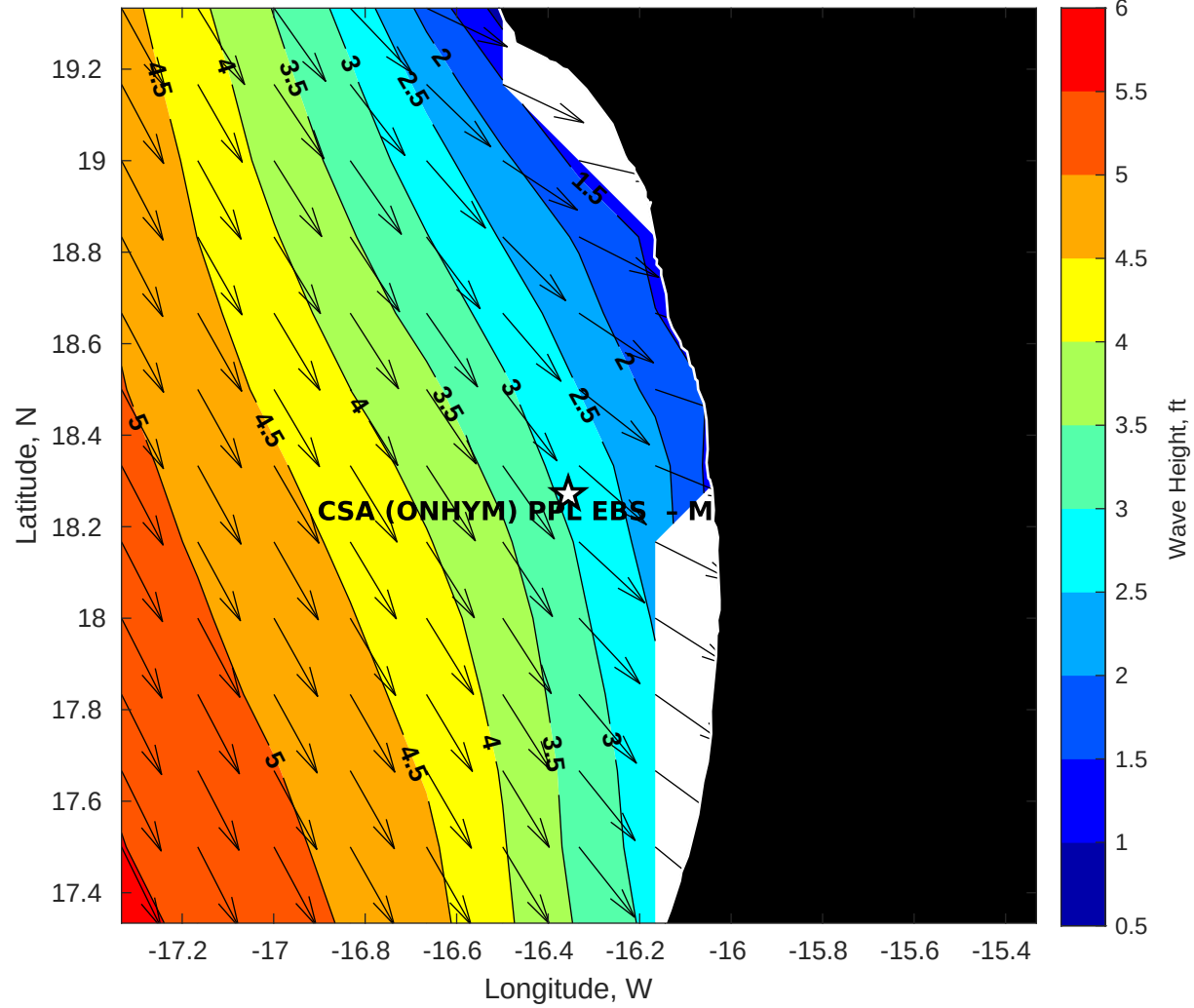
GFS Wave Height (ft) for CSA (ONHYM) PPL EBS - Mauritania at 27-Jan-2026 09:00:00
