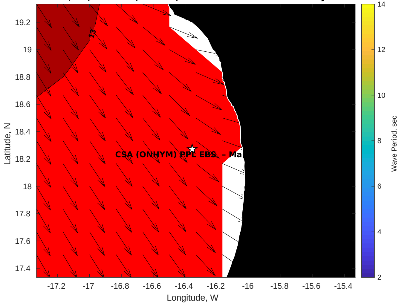
GFS Wave Period (sec) for CSA (ONHYM) PPL EBS - Mauritania at 27-Jan-2026 09:00:00
