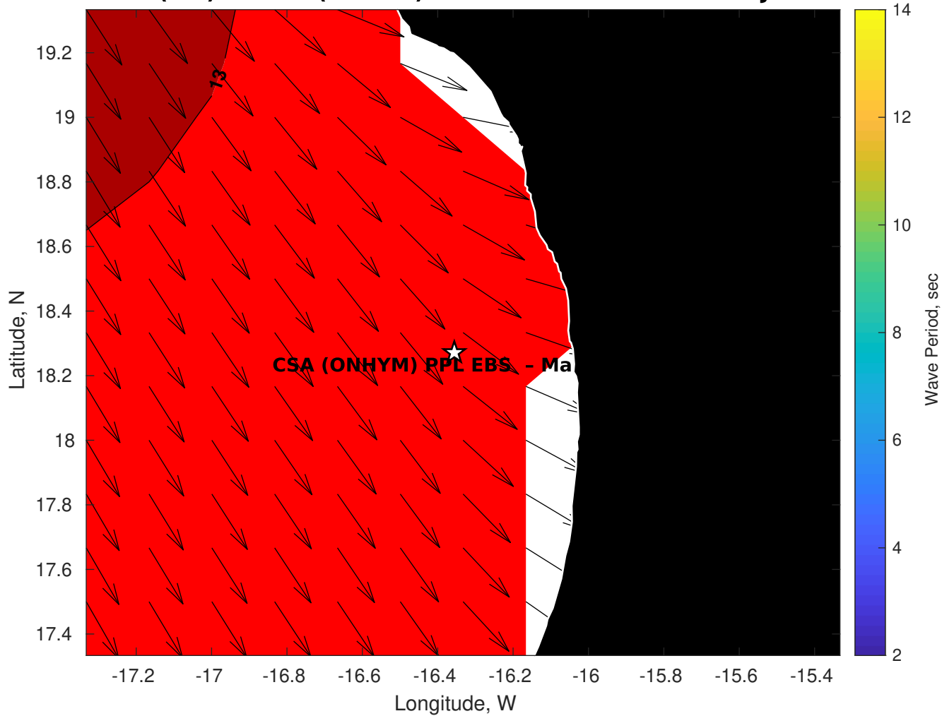
GFS Wave Period (sec) for CSA (ONHYM) PPL EBS - Mauritania at 27-Jan-2026 09:00:00
