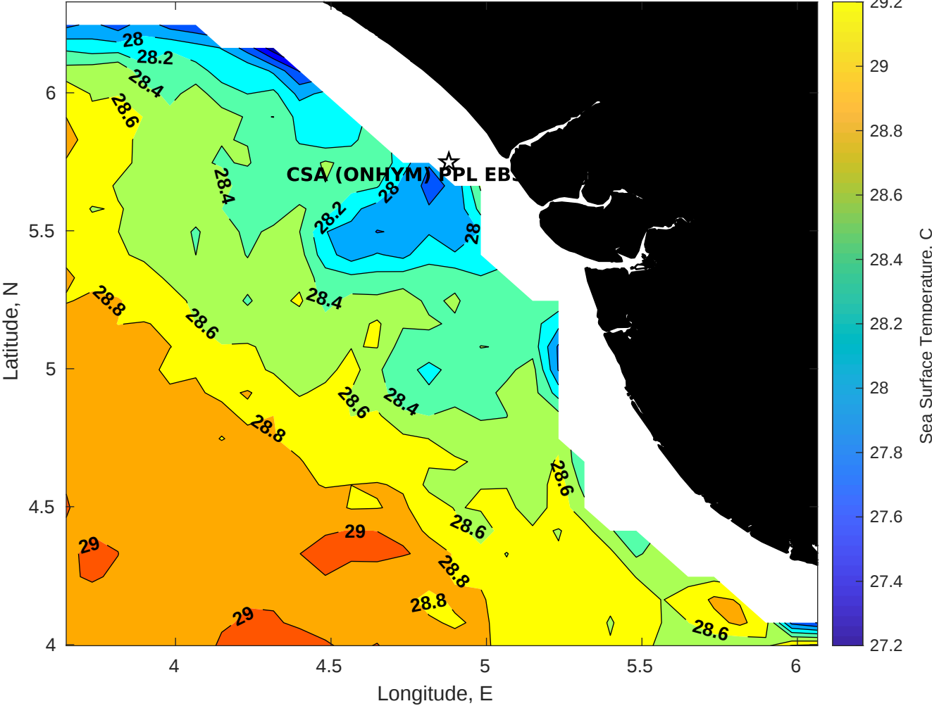
SST for CSA (ONHYM) PPL EBS - Nigeria at 26-Jan-2026 00:00:00
