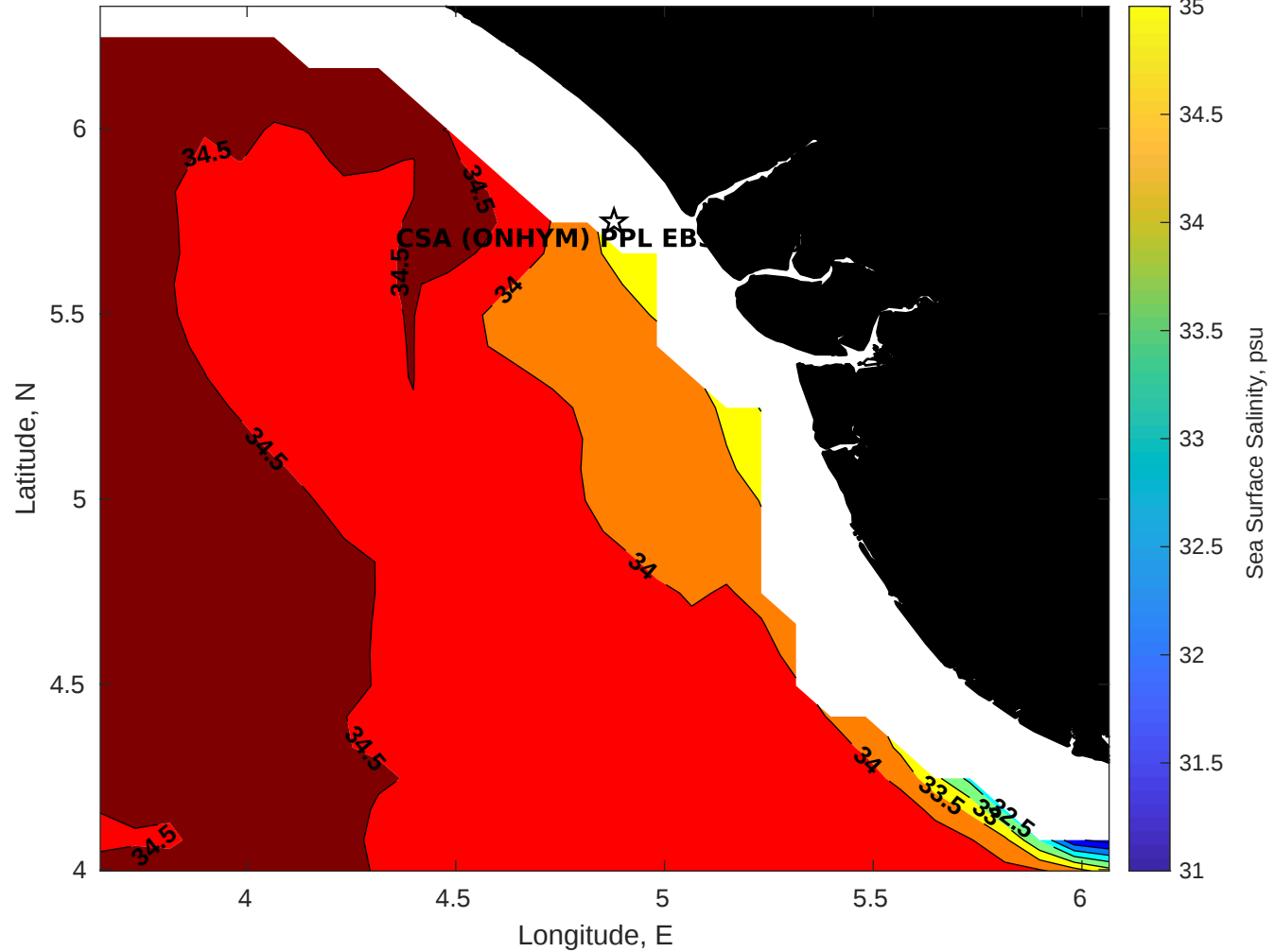
Surface Salinity for CSA (ONHYM) PPL EBS - Nigeria at 26-Jan-2026 00:00:00
