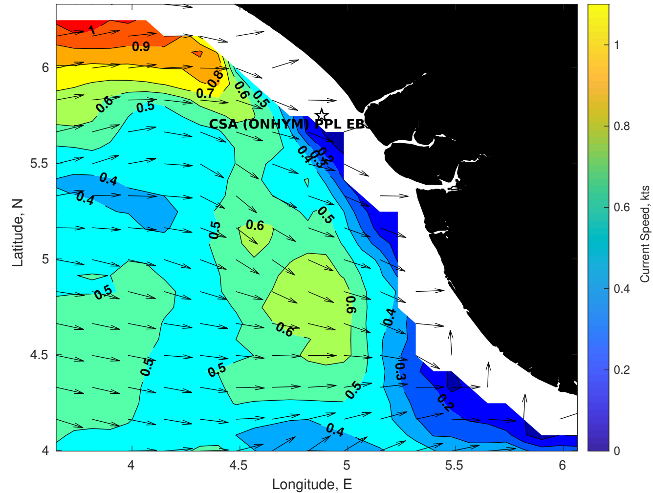
Surface Currents for CSA (ONHYM) PPL EBS - Nigeria at 26-Jan-2026 00:00:00
