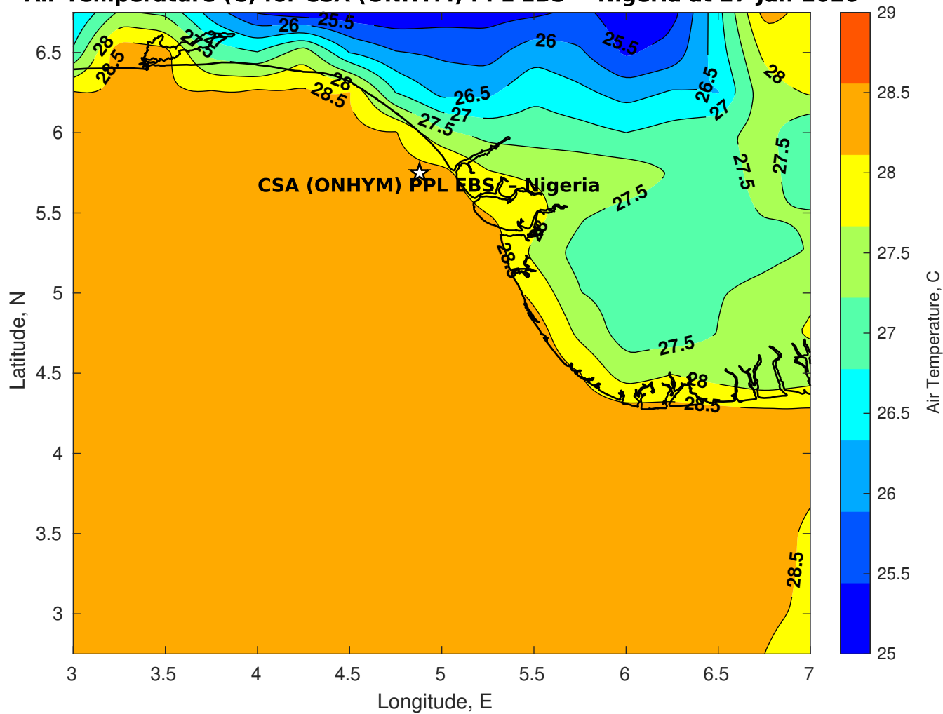
Air Temperature (C) for CSA (ONHYM) PPL EBS - Nigeria at 27-Jan-2026
