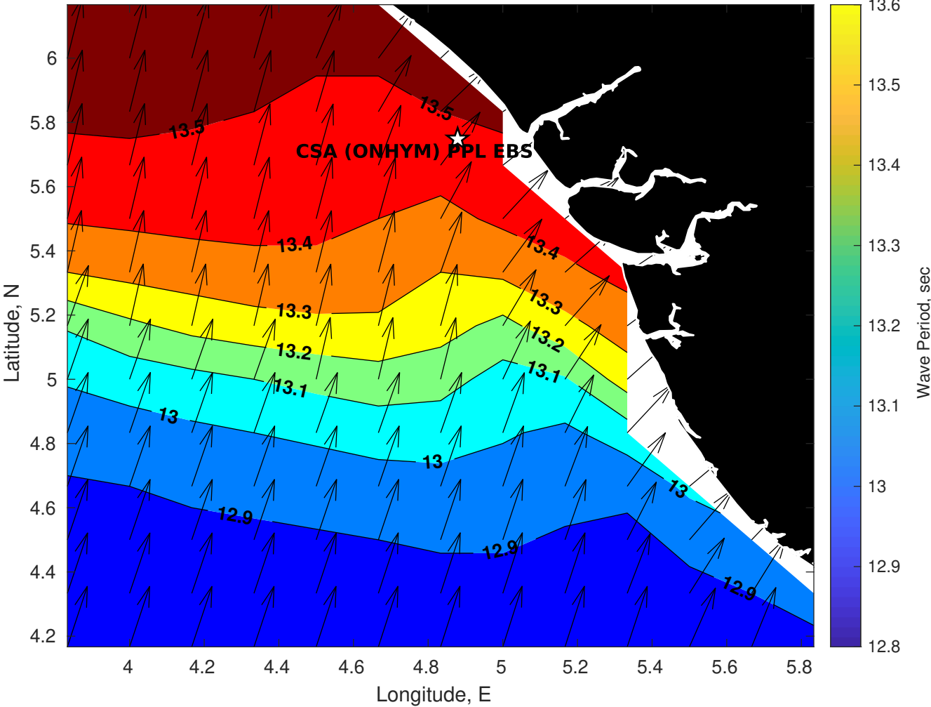
GFS Wave Period (sec) for CSA (ONHYM) PPL EBS - Nigeria at 27-Jan-2026 09:00:00
