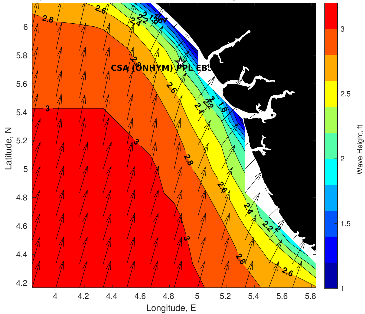
GFS Wave Height (ft) for CSA (ONHYM) PPL EBS - Nigeria at 27-Jan-2026 09:00:00
