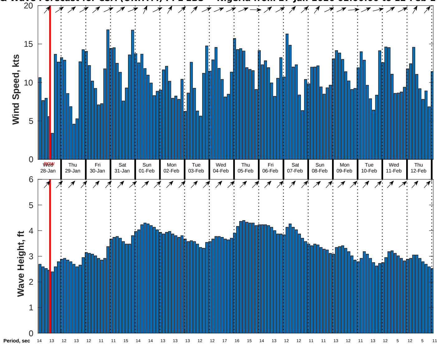
Wind & Wave Forecast for CSA (ONHYM) PPL EBS - Nigeria from 27-Jan-2026 02:00:00 to 12-Feb-2026 02:00:00
