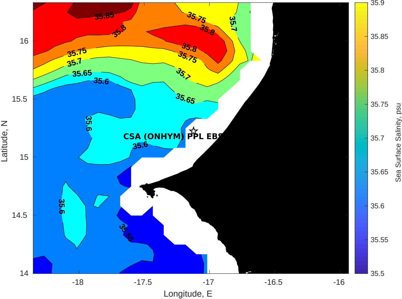
Surface Salinity for CSA (ONHYM) PPL EBS - Senegal at 26-Jan-2026 00:00:00
