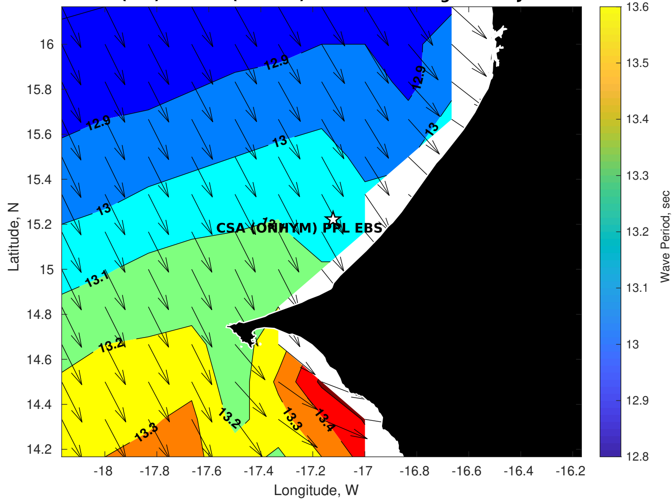
GFS Wave Period (sec) for CSA (ONHYM) PPL EBS - Senegal at 27-Jan-2026 09:00:00
