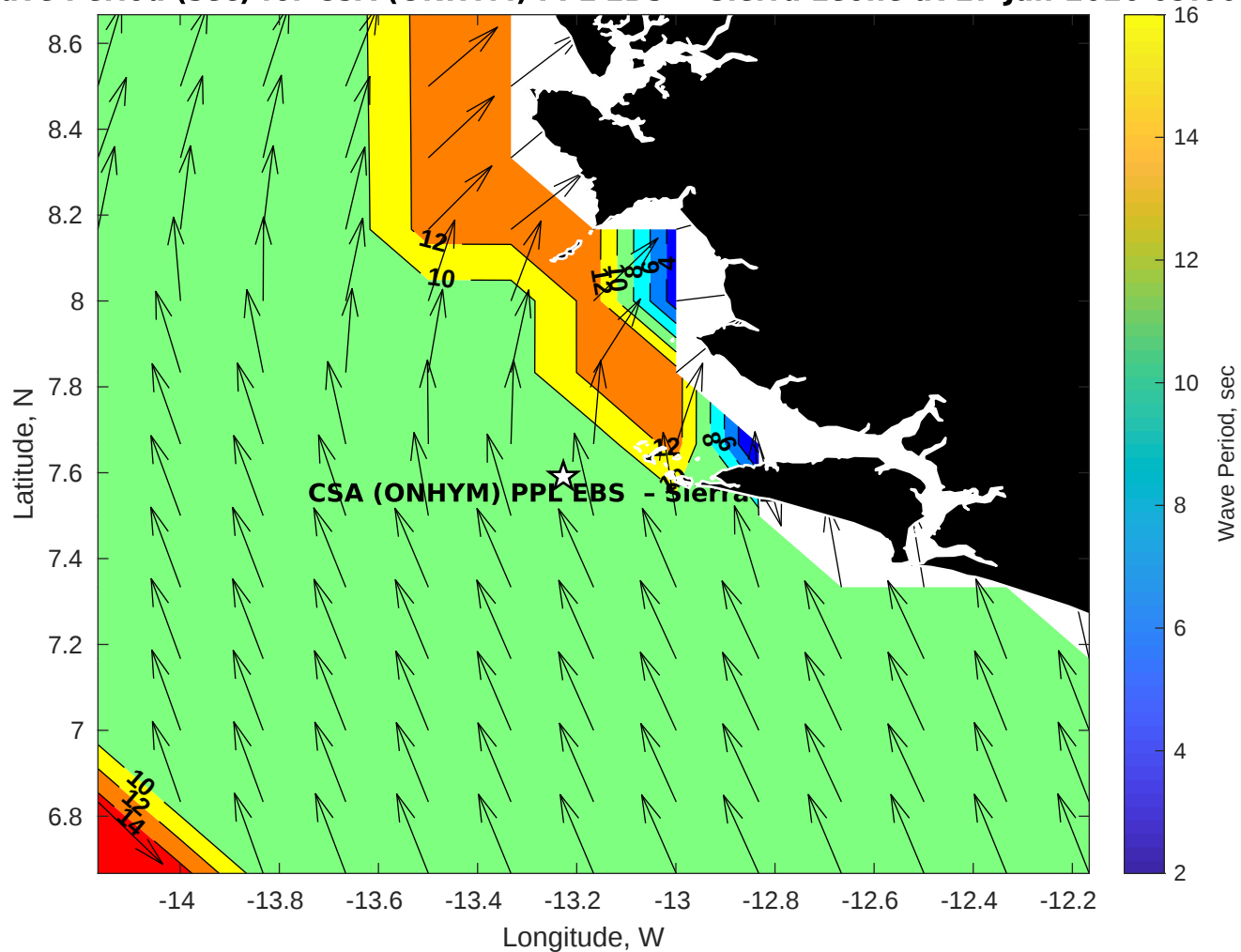
GFS Wave Period (sec) for CSA (ONHYM) PPL EBS - Sierra Leone at 27-Jan-2026 09:00:00
