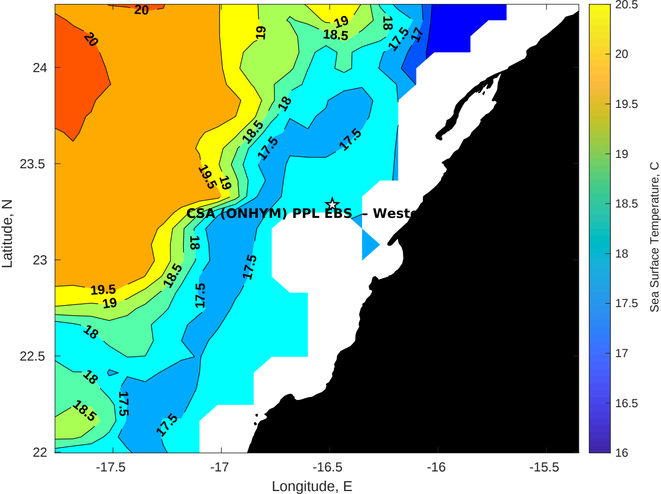
SST for CSA (ONHYM) PPL EBS - Western Sahara at 26-Jan-2026 00:00:00
