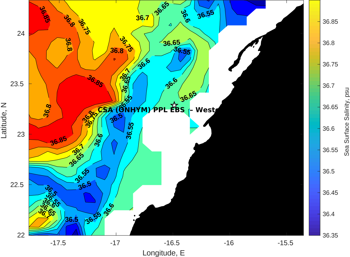
Surface Salinity for CSA (ONHYM) PPL EBS - Western Sahara at 26-Jan-2026 00:00:00
