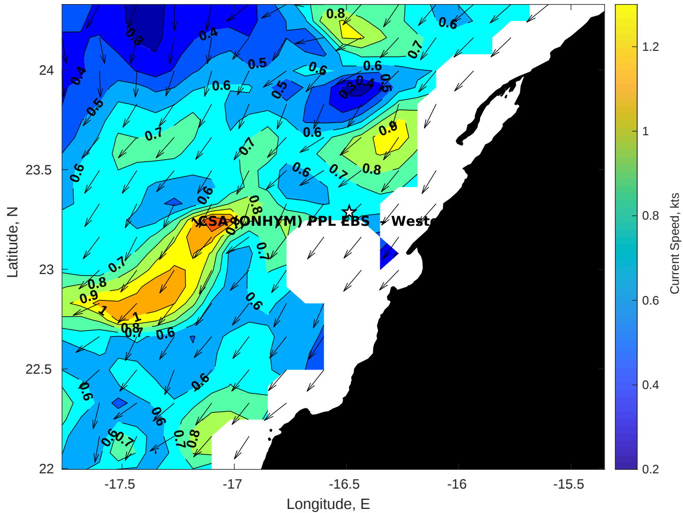
Surface Currents for CSA (ONHYM) PPL EBS - Western Sahara at 26-Jan-2026 00:00:00
