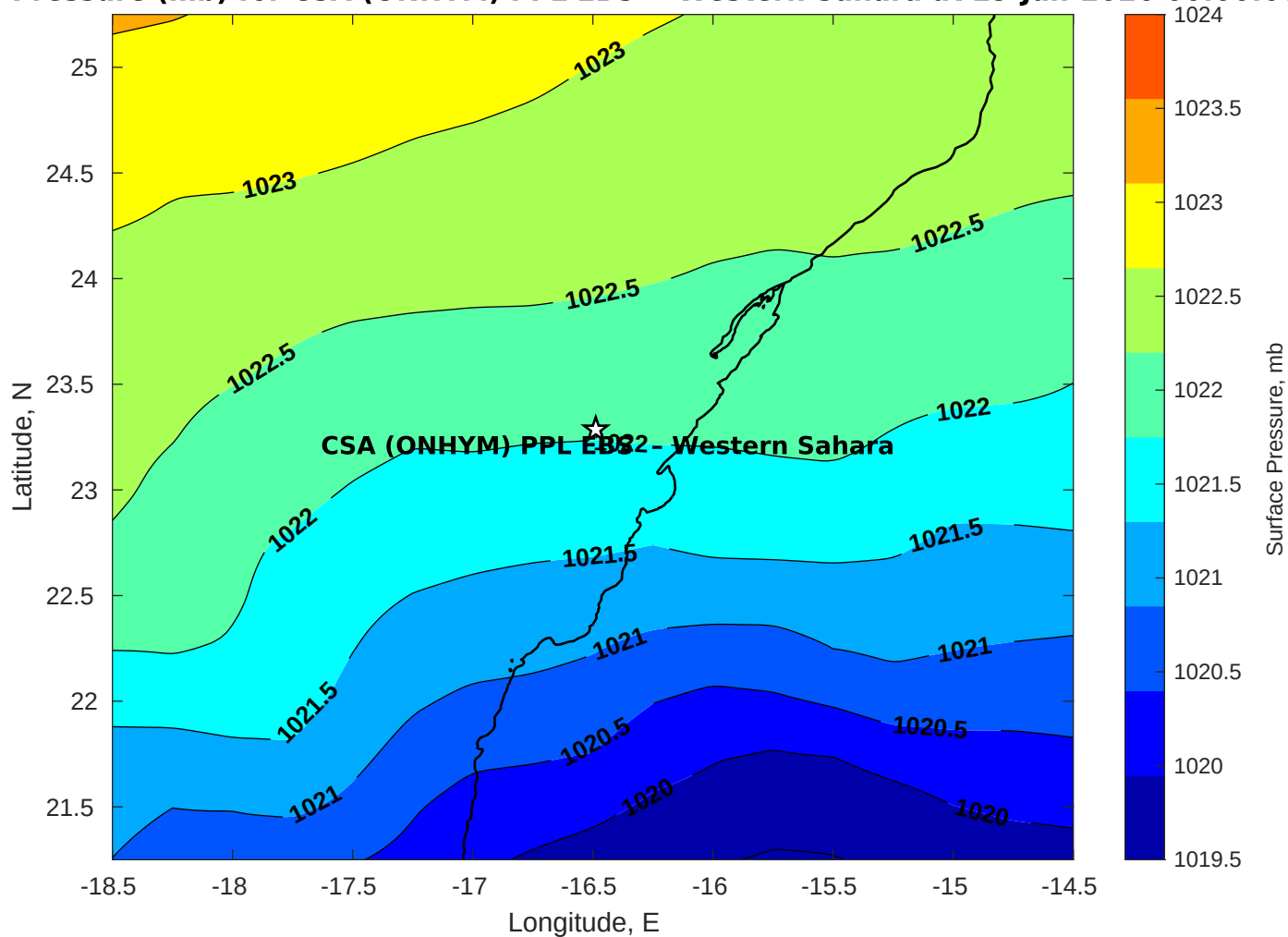
Surface Pressure (mb) for CSA (ONHYM) PPL EBS - Western Sahara at 29-Jan-2026 00:00:00
