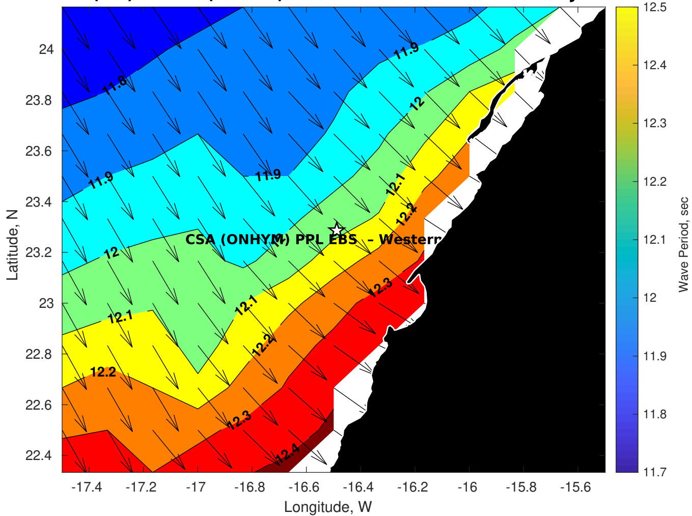
GFS Wave Period (sec) for CSA (ONHYM) PPL EBS - Western Sahara at 27-Jan-2026 09:00:00
