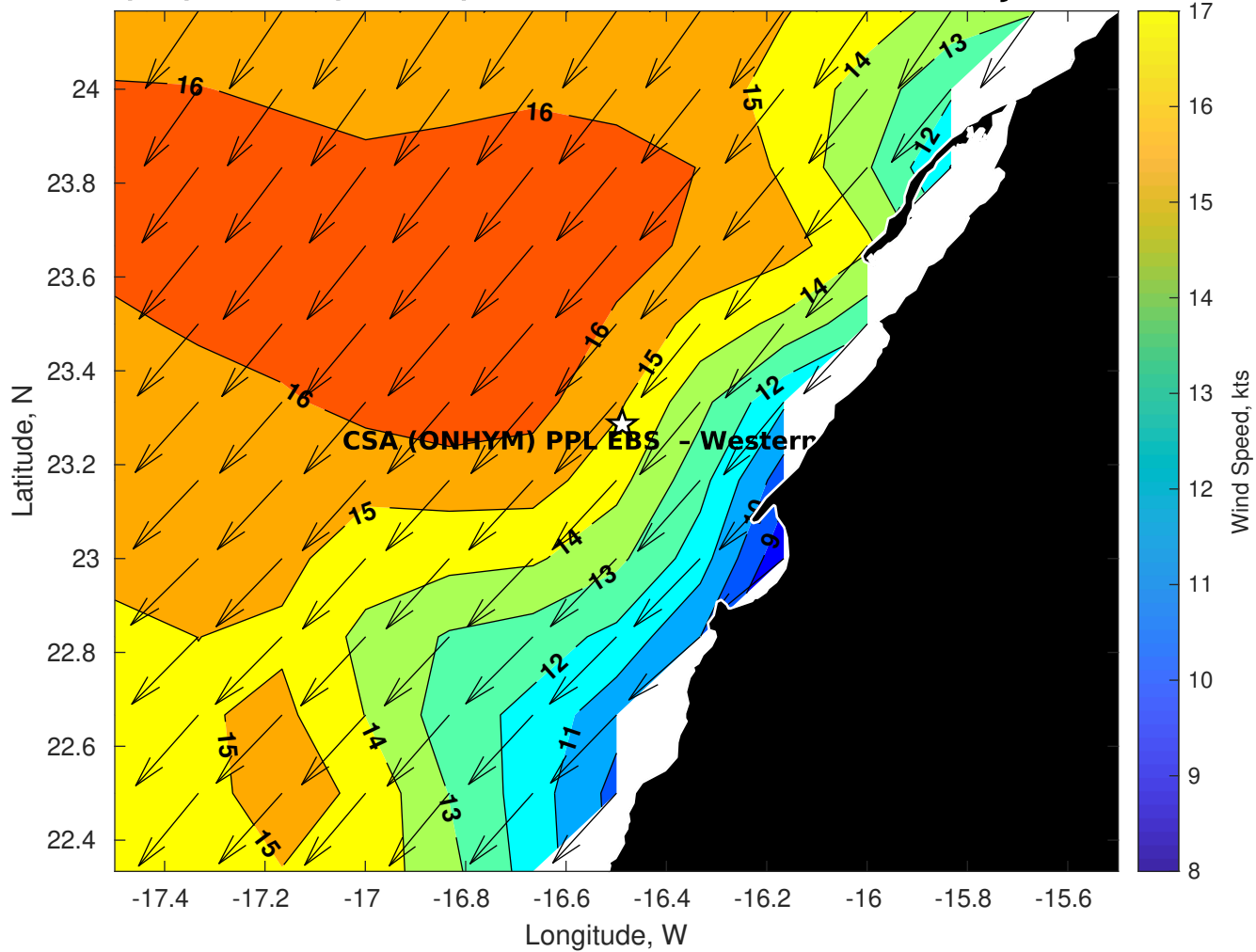
GFS Winds (kts) for CSA (ONHYM) PPL EBS - Western Sahara at 27-Jan-2026 09:00:00
