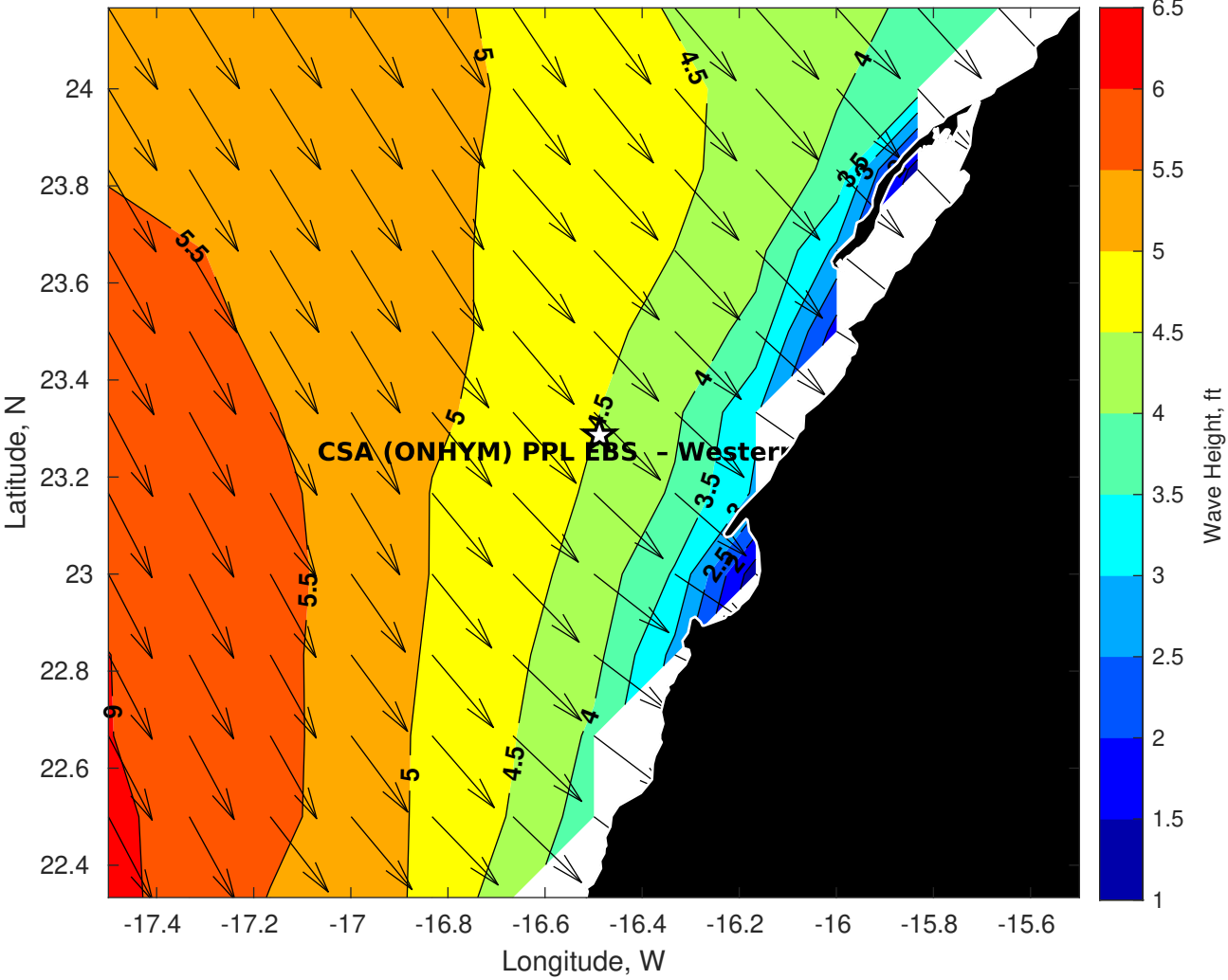
GFS Wave Height (ft) for CSA (ONHYM) PPL EBS - Western Sahara at 27-Jan-2026 09:00:00
