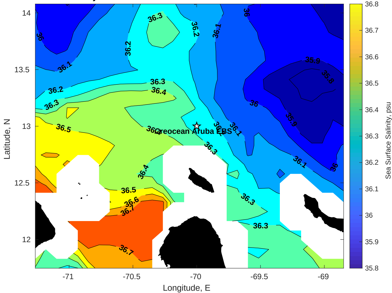
Surface Salinity for Creoccean Aruba EBS at 26-Jan-2026 00:00:00
