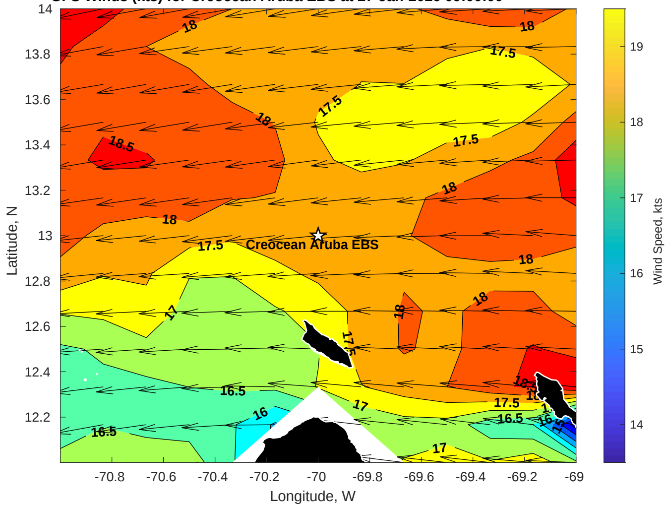
GFS Winds (kts) for Creoccean Aruba EBS at 27-Jan-2026 09:00:00
