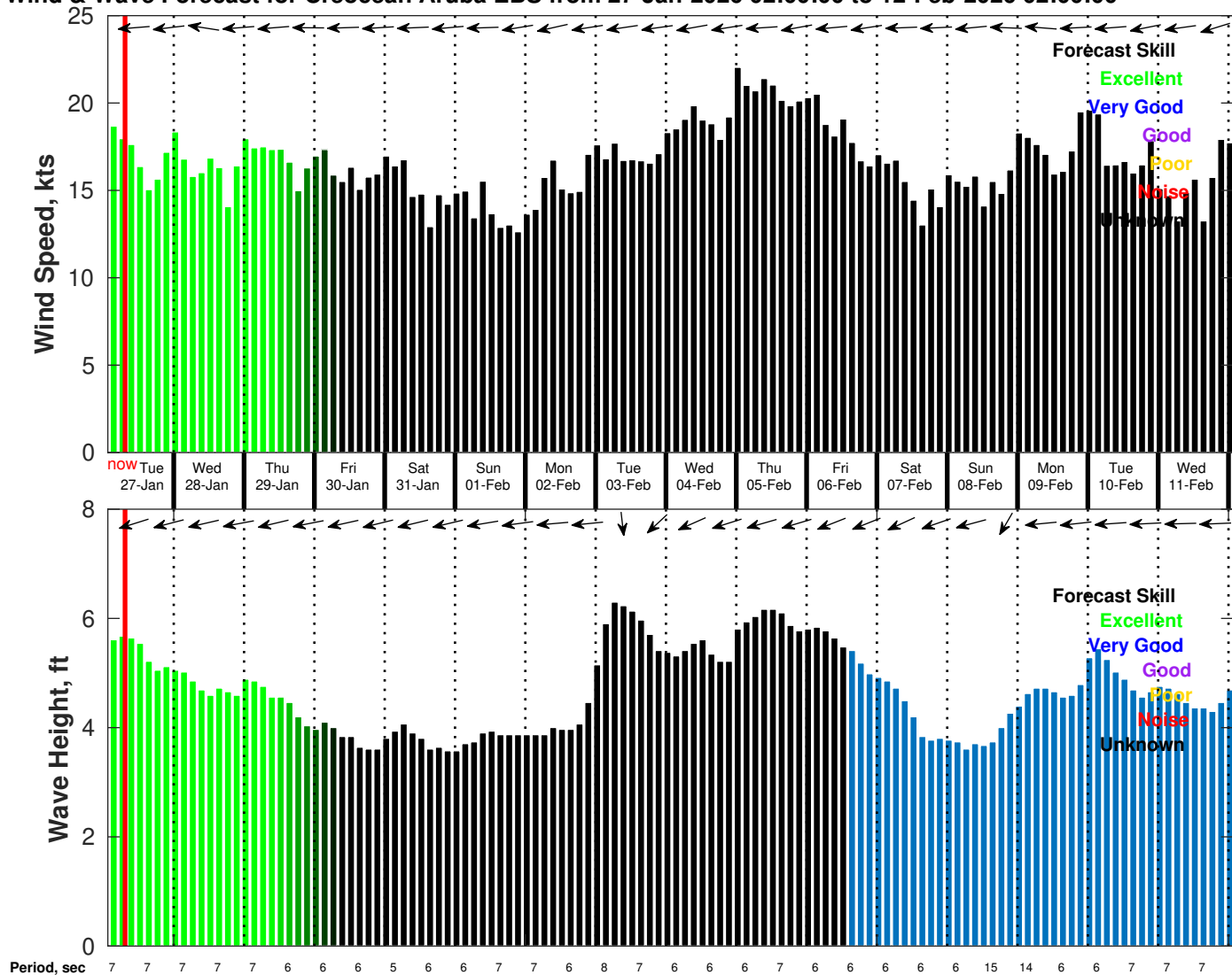
Wind & Wave Forecast for Creocan Aruba EBS from 27-Jan-2026 02:00:00 to 12-Feb-2026 02:00:00
