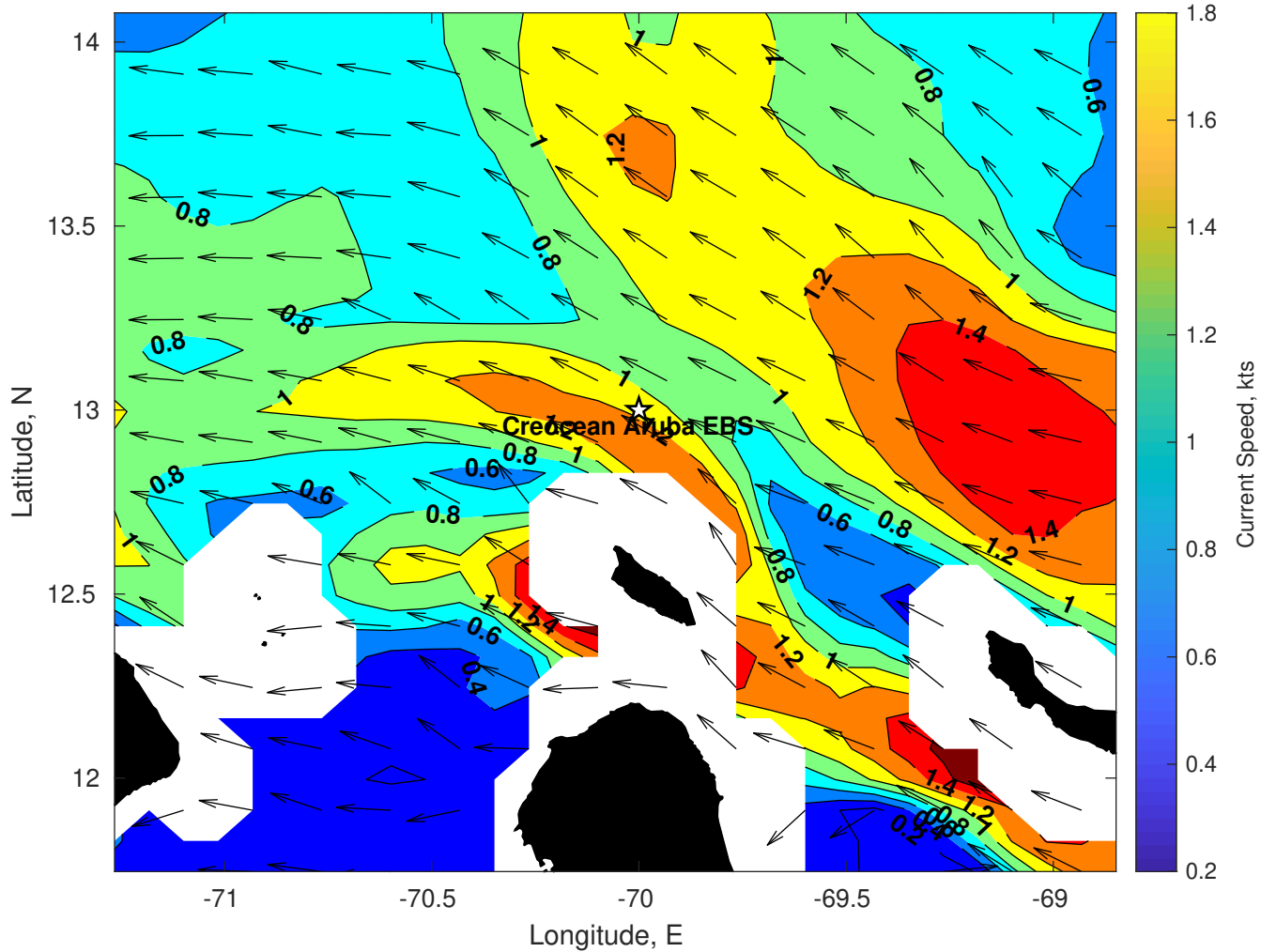
Surface Currents for Creocan Aruba EBS at 26-Jan-2026 00:00:00
