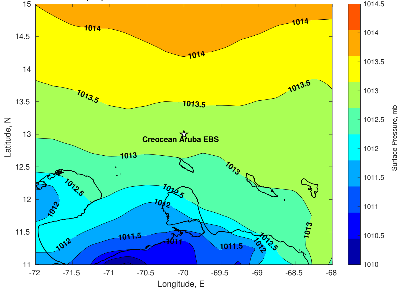
Surface Pressure (mb) for Creoccean Aruba EBS at 28-Jan-2026 18:00:00
