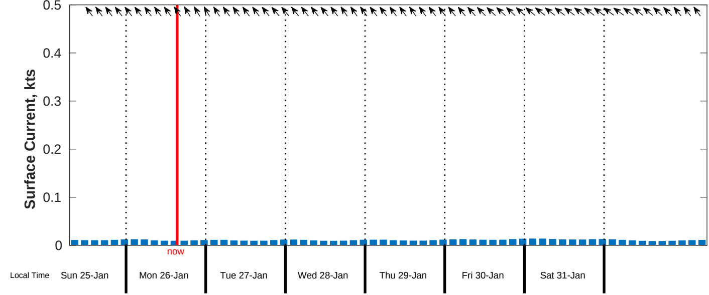
Surface Current Forecast for Creocean Aruba EBS from 26-Jan-2026 00:00:00 to 03-Feb-2026 00:00:00
