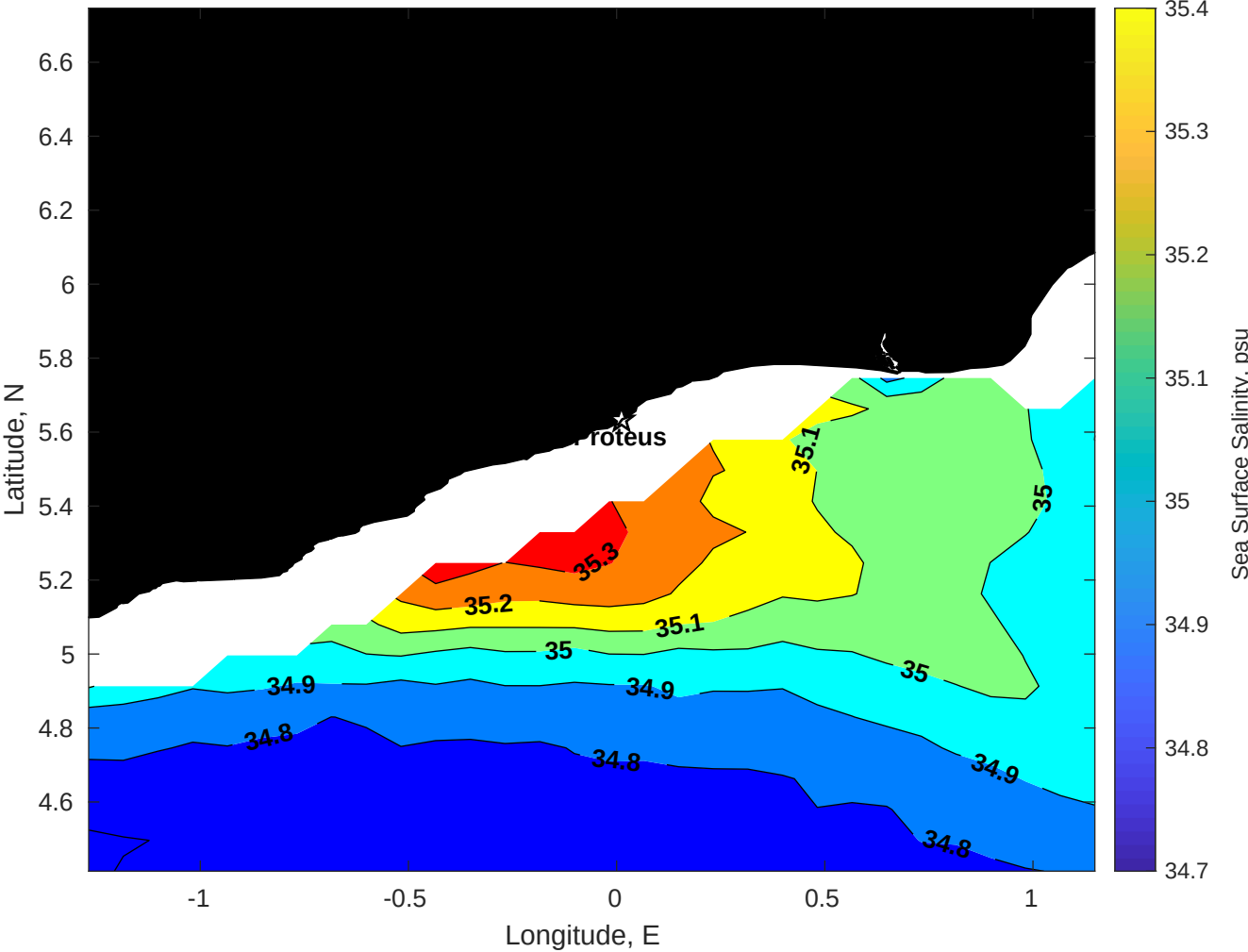
Surface Salinity for Proteus at 26-Jan-2026 00:00:00
