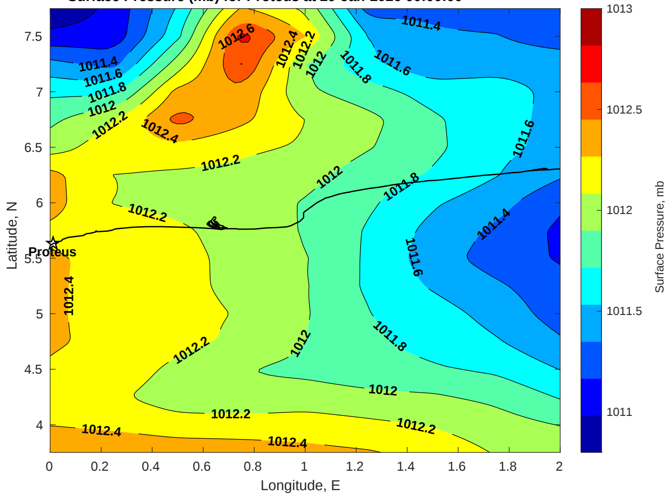
Surface Pressure (mb) for Proteus at 29-Jan-2026 00:00:00
