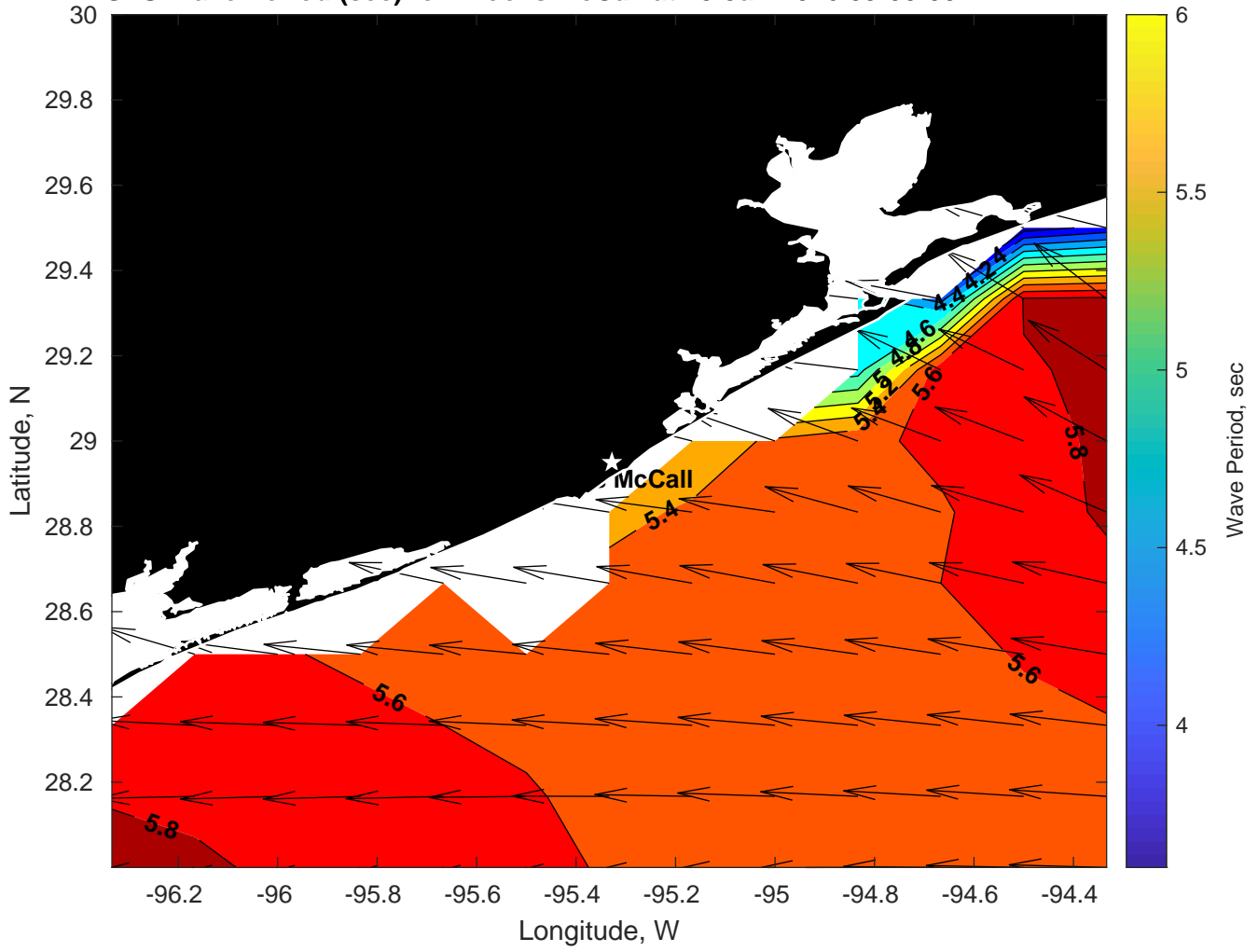
GFS Wave Period (sec) for Brooks McCall at 28-Jan-2026 09:00:00
