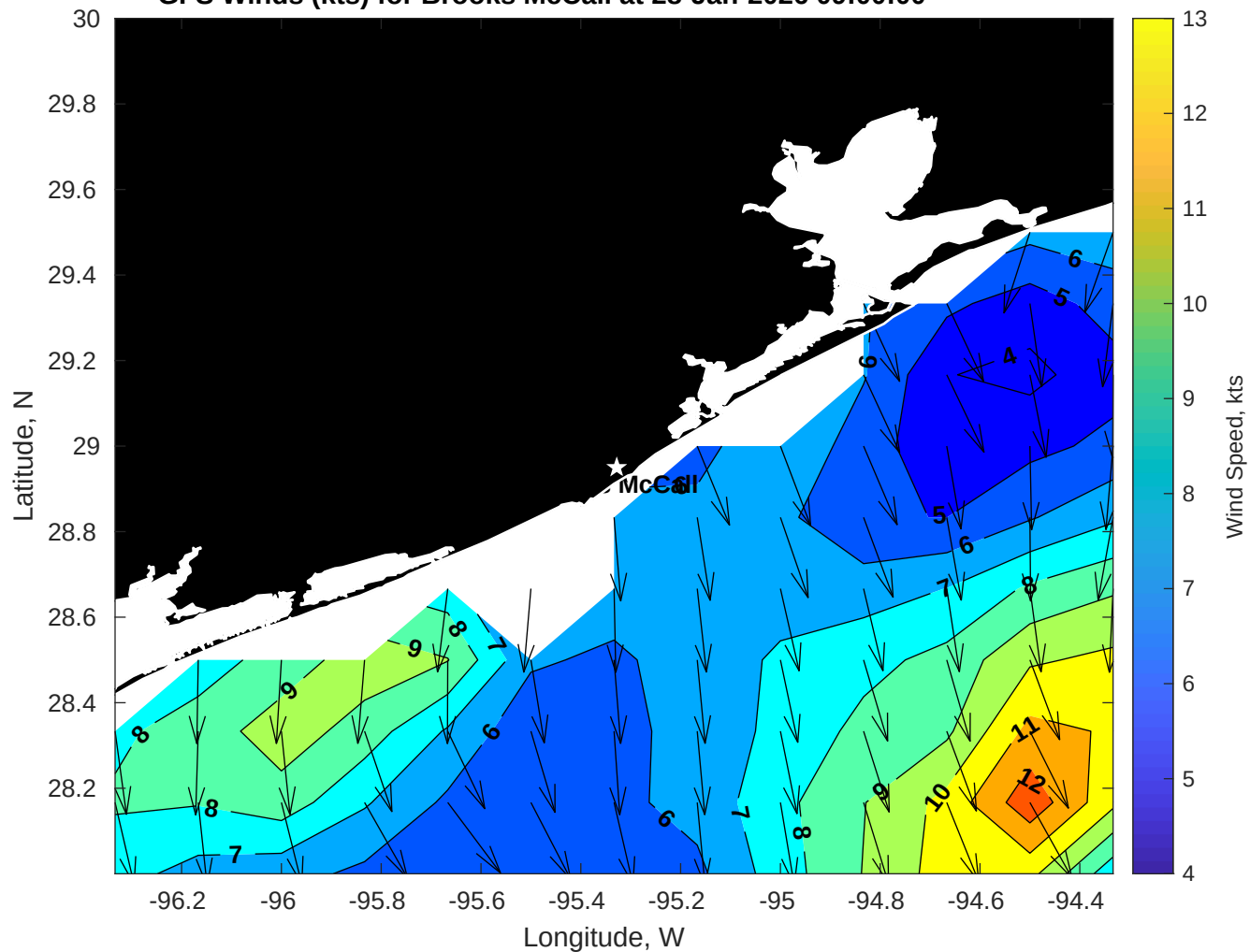
GFS Winds (kts) for Brooks McCall at 28-Jan-2026 09:00:00
