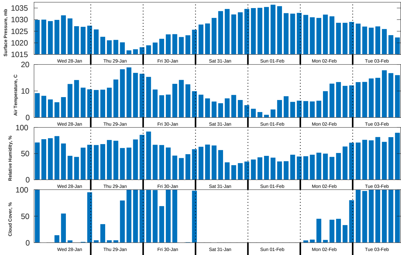
Met Forecast for Brooks McCall from 28-Jan-2026 00:00:00 to 04-Feb-2026 00:00:00
