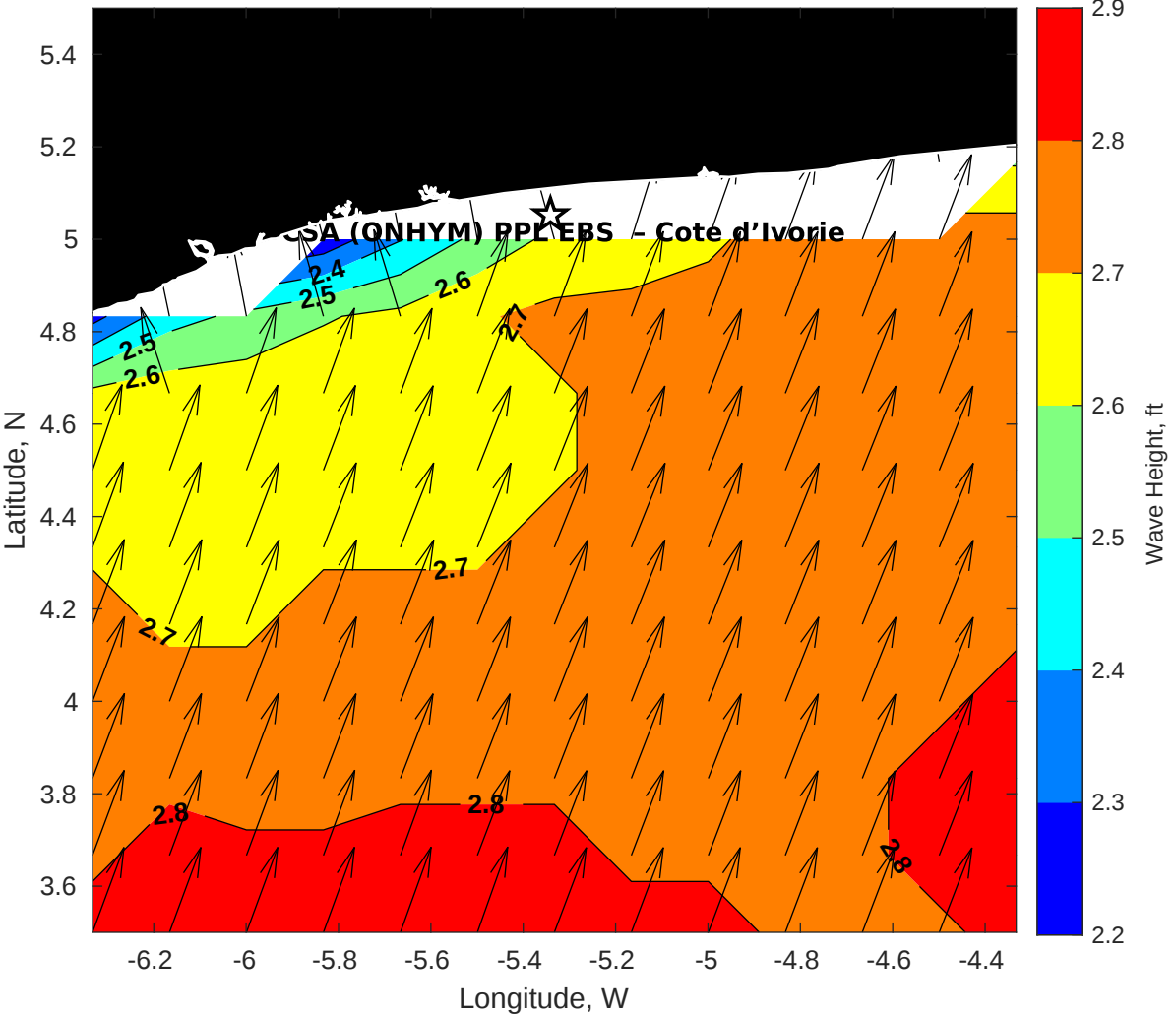
GFS Wave Height (ft) for CSA (ONHYM) PPL EBS - Cote d'Ivoire at 28-Jan-2026 09:00:00
