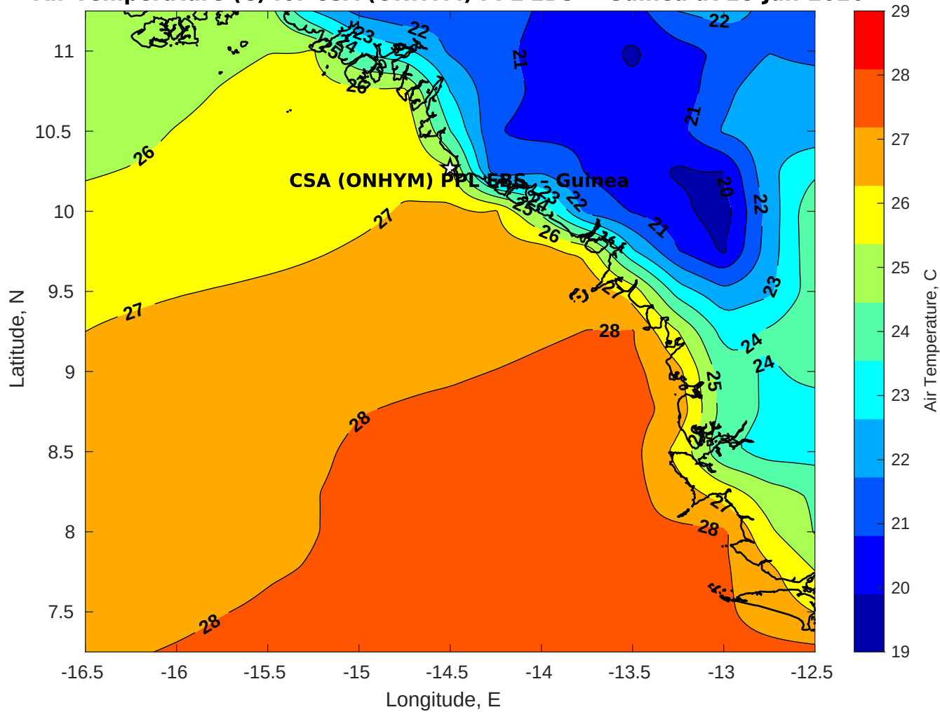
Air Temperature (C) for CSA (ONHYM) PPL EBS - Guinea at 28-Jan-2026
