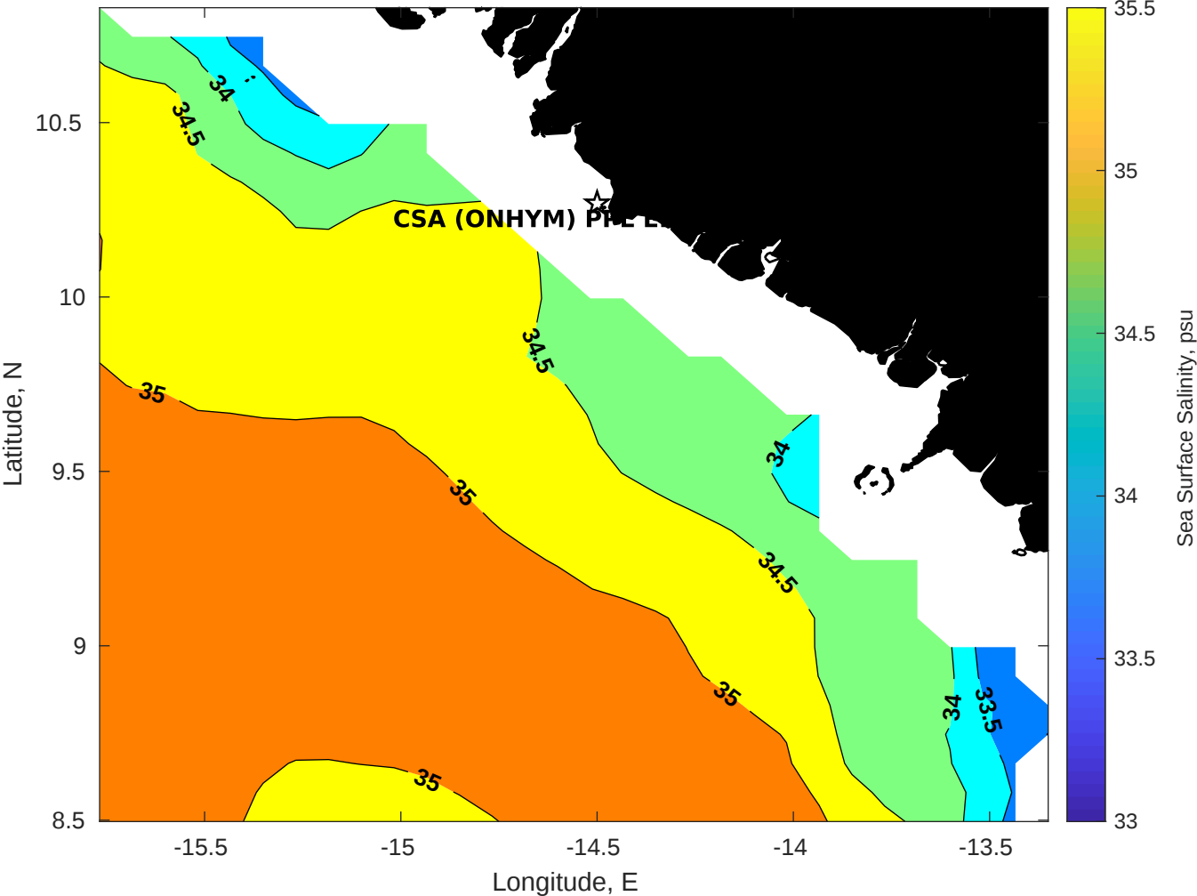
Surface Salinity for CSA (ONHYM) PPL EBS - Guinea at 27-Jan-2026 00:00:00
