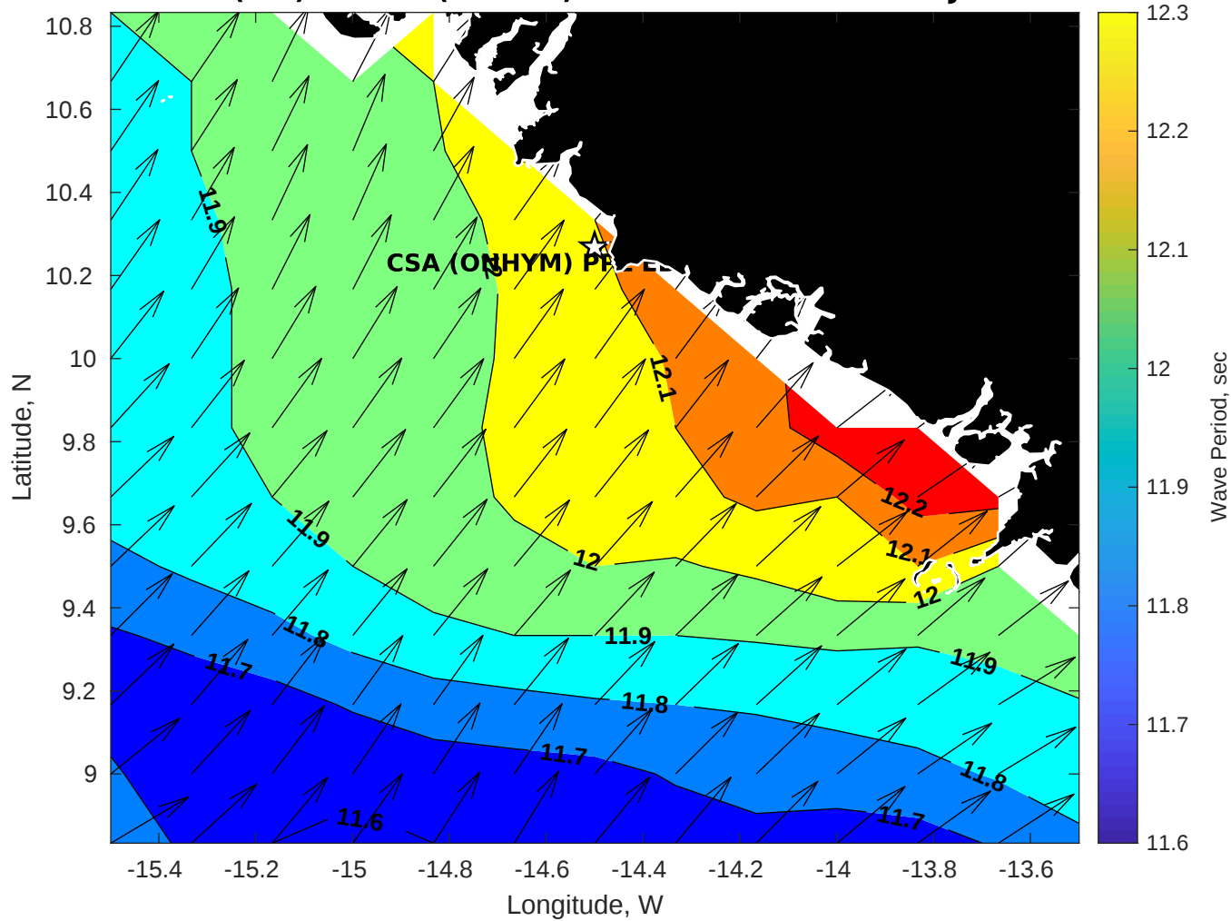
GFS Wave Period (sec) for CSA (ONHYM) PPL EBS - Guinea at 28-Jan-2026 09:00:00
