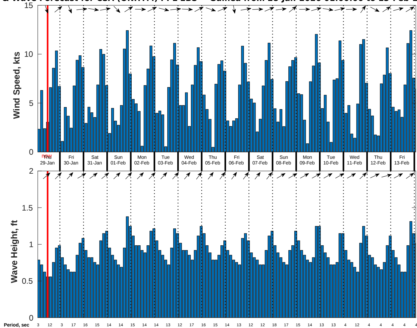
Wind & Wave Forecast for CSA (ONHYM) PPL EBS - Guinea from 28-Jan-2026 01:00:00 to 13-Feb-2026 01:00:00
